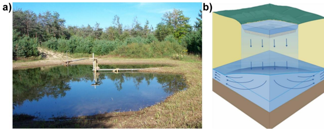
Figure 83 - Rapid infiltration basins (RIBs) have been tested successfully across parts of the Oak Ridges Moraine aquifer in southern Ontario, Canada. a) A recharge pond. b) Schematic of flow from the pond to the underlying water table with a mound developing below the pond (from Howard et al., 2000, 2007; photography by Ken Howard).
