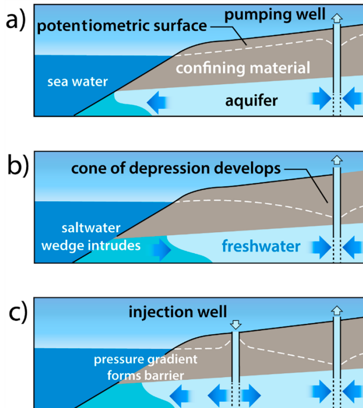
Figure 63 - To stop the advance of seawater, sets of closely spaced wells were drilled in Los Angeles to inject high-quality freshwater into the aquifer, thus creating hydraulic pressure ridges or barriers (USGS, 2018).
