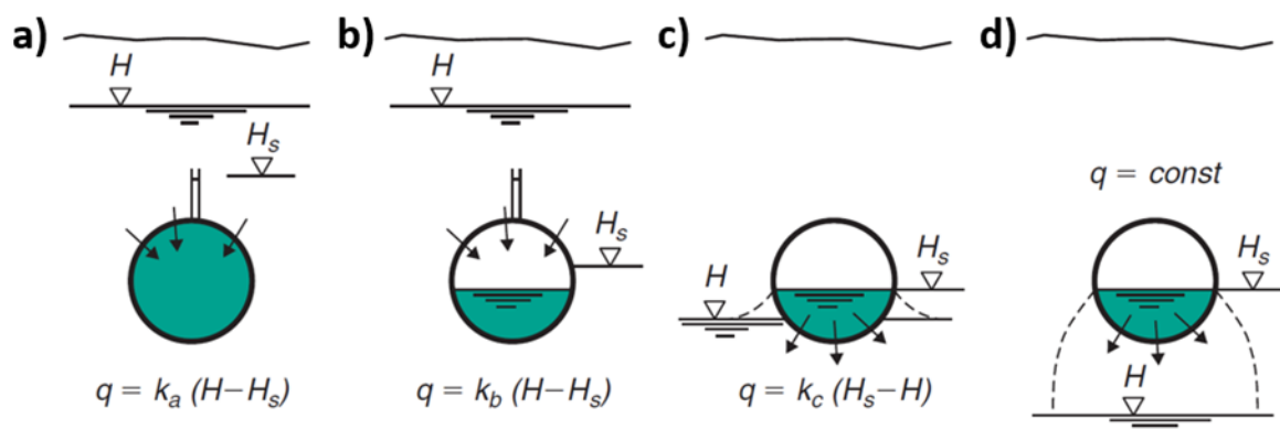
Figure 18 - Formulas for calculating sewer infiltration rates a) and b) and exfiltration rates c) and d) for typical water table conditions (a) and b) after Mills and others, 2014; c) and d) after Pokrajac & Howard, 2010).
