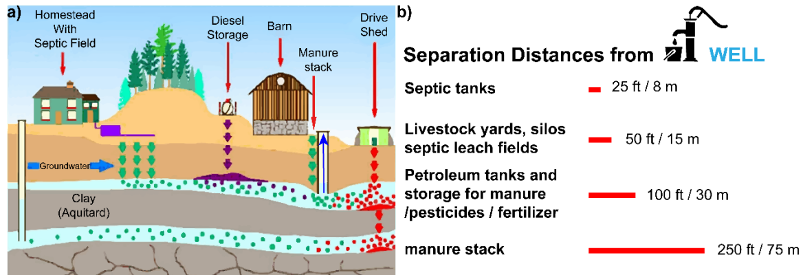
Figure 93 - The simplest standards of practice approach involves establishing minimum separation distances (setbacks) between a potential contaminant source and the water supply such as a well or spring (from a) Ontario Ministry of Environment, Conservation, and Parks, 2023; b) figure by Ken Howard).
