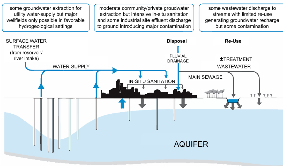
Figure 56 - Unconfined groundwater and its interaction with urban infrastructure and wastewater in cities of many low- and middle-income countries. A combination of local community/private extraction and intensive in-situ sanitation often leads to serious groundwater contamination issues (after Foster et al., 2010b).
