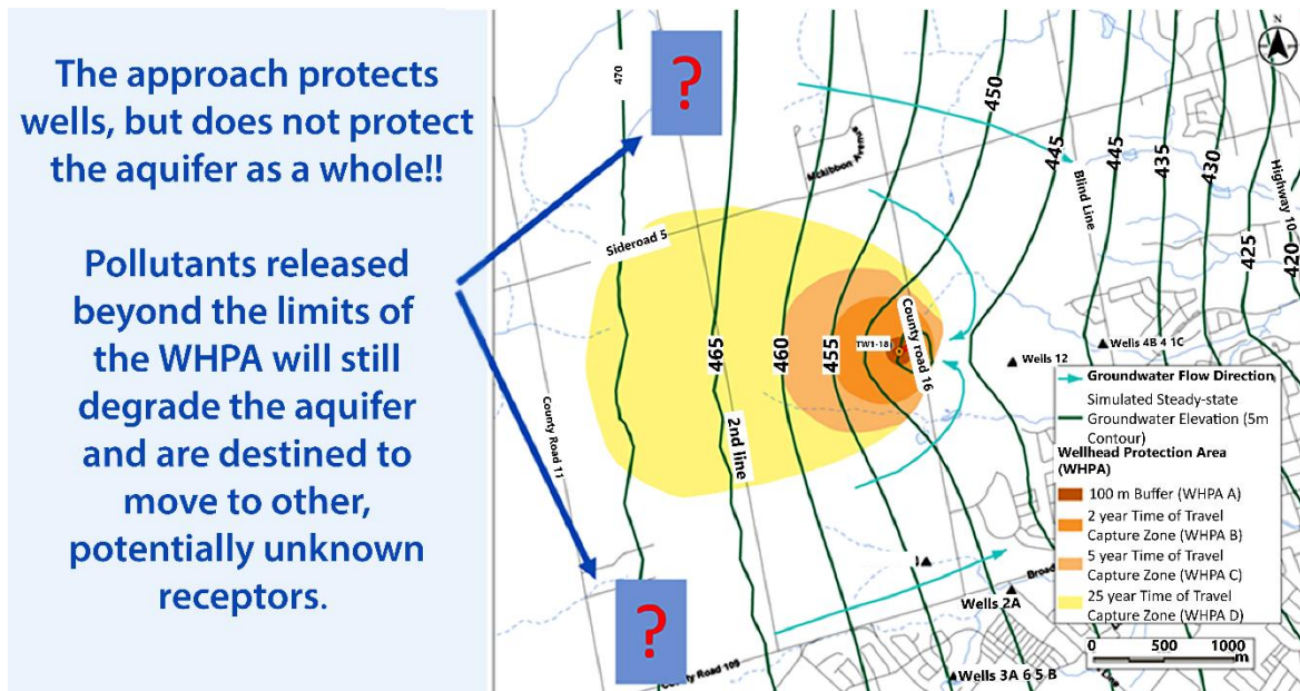
Figure 103 - The WHPA/SPZ/ZOC technique focuses on the protection of individual wells and can be effective for those wells if reliably delimited and the flow field remains stable over time. The practice of excluding potential sources of groundwater contamination from the protected area will inevitably increase the risk of groundwater contamination in the remaining “unprotected” parts of the aquifer (figure by Ken Howard).
