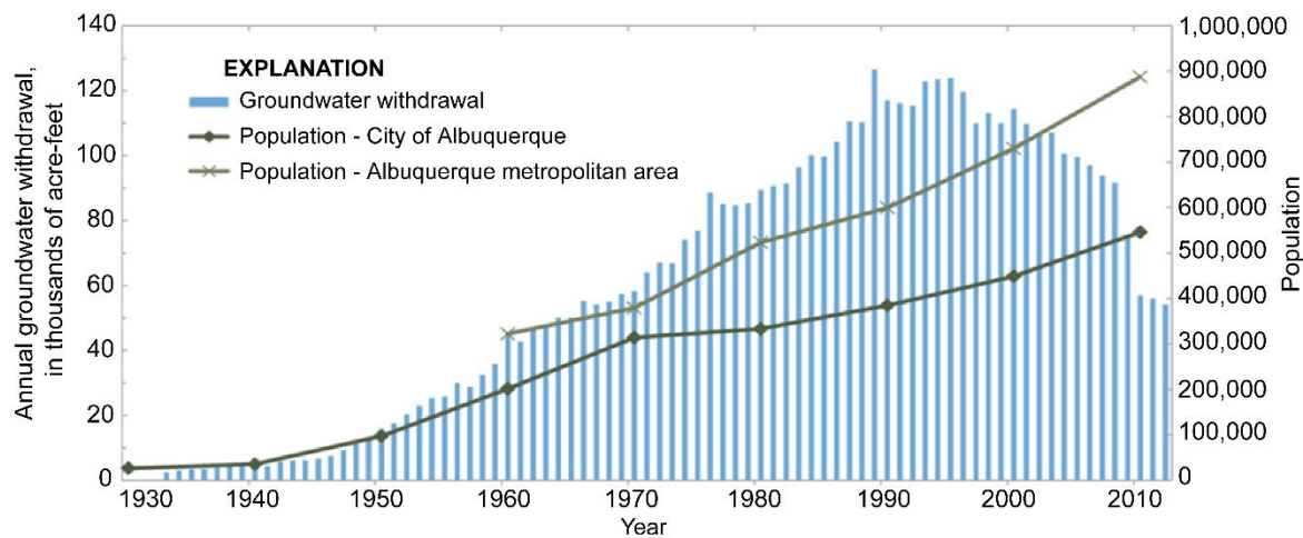
Figure 23 - In Albuquerque, New Mexico, USA, a rapidly growing population led to over-exploitation of groundwater reserves, which led to a 50 percent reduction in groundwater withdrawals from the city’s aquifer. The city’s strategy for water supply now involves the conjunctive use of groundwater and surface water (Turin et al., 1997).
