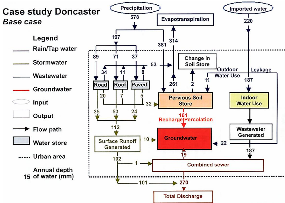
Figure 111 - Urban water balance determined using the UVQ for the City of Doncaster, England (after Wolf et al., 2006).
