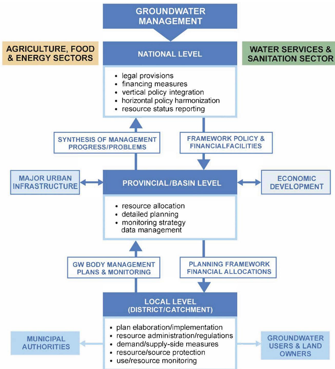
Figure 126 - Broad scheme of governance provisions required for vertical integration and horizontal coordination of groundwater management (modified after Foster & van der Gun, 2016).
