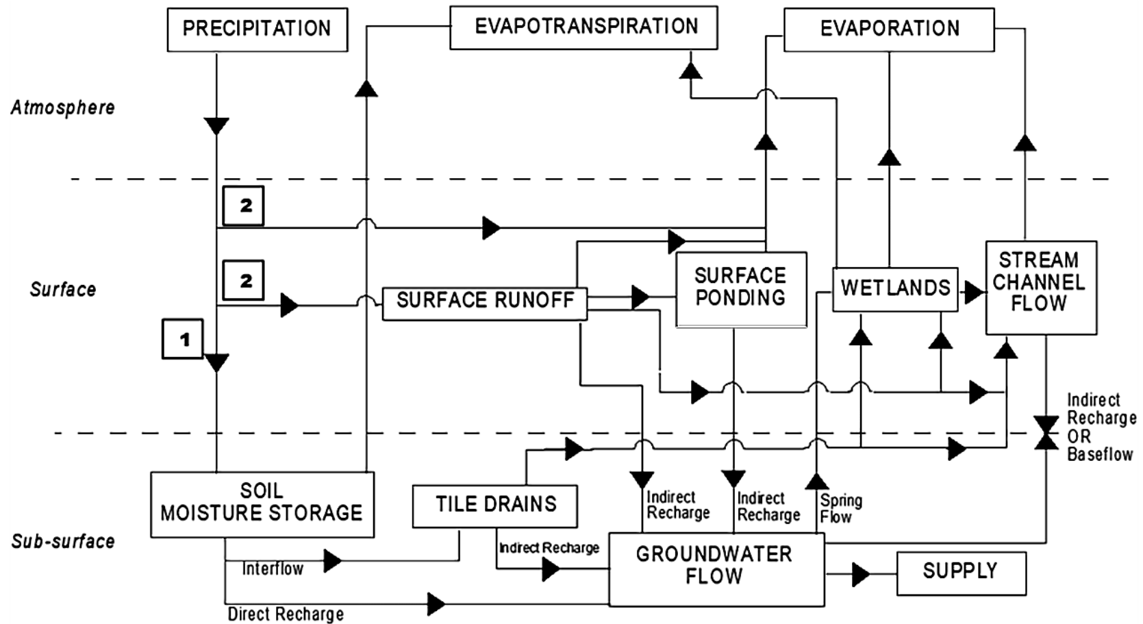
Figure 8 - Preferred water flow paths in urban areas. Pathway 1 (leading to direct recharge) is the preferred route for precipitation that falls on vegetated surfaces. Direct recharge refers to water that infiltrates into the soil soon after its arrival as incident precipitation (Howard & Lloyd, 1979) and passes directly to the underlying aquifer in approximately the location where it falls. Pathway 2 (leading to indirect recharge) is the route for precipitation that encounters impermeable surfaces. Indirect recharge normally occurs when water infiltrates following transport across the land surface as runoff. It most commonly occurs in vegetated swales, stream channels or beneath shallow temporary ponds that form following intense periods of rain (Howard, 1997).
