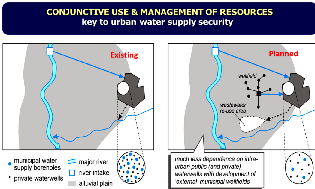
Figure 130 - Example of a conjunctive use scheme for urban water supply (modified after Foster et al., 2010d).
