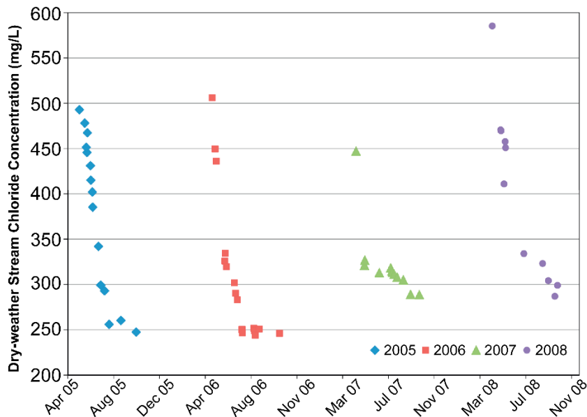
Figure 53 - Chloride concentrations in baseflow at the Highland Creek monitoring station on Morningside Avenue (Toronto, Canada) under non-winter, dry-weather flow conditions, which are generally April through August. During these conditions, we can assume the flow of water in the channel is entirely represented by groundwater discharge, that is, baseflow (after Perera et al., 2013).
