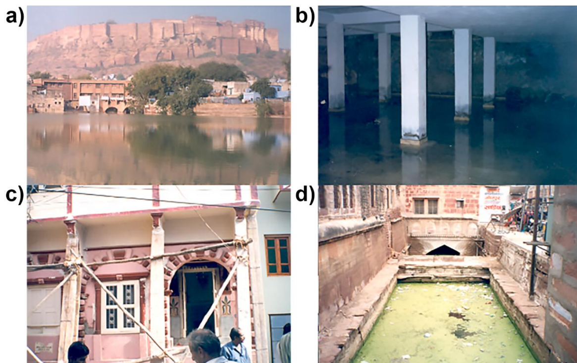
Figure 26 - In Jodhpur, India, groundwater levels were found to be rising 1 to 1.5 m per year despite persistent drought conditions. a) Gulab Sagar Lake remains filled with water even in the summer, b) basements flood, c) house foundations in the old city are damaged, and d) Gorinda Bauri (an old step well) overflows (after Paliwal & Baghela, 2007). The problem was caused by construction of the Indira Gandhi Canal, which brought water into the city from the Himalayas. Leakage from the canal, poor drainage, leaking sewers, and the abandonment of local dug wells, step wells, and pond supplies all contributed to the problem (photography by B.S. Paliwal and A. Baghela).
