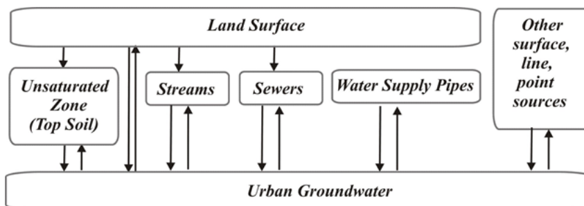
Figure 114 - Interaction between control volumes in the urban water balance (Pokrajac and Howard, 2010).
