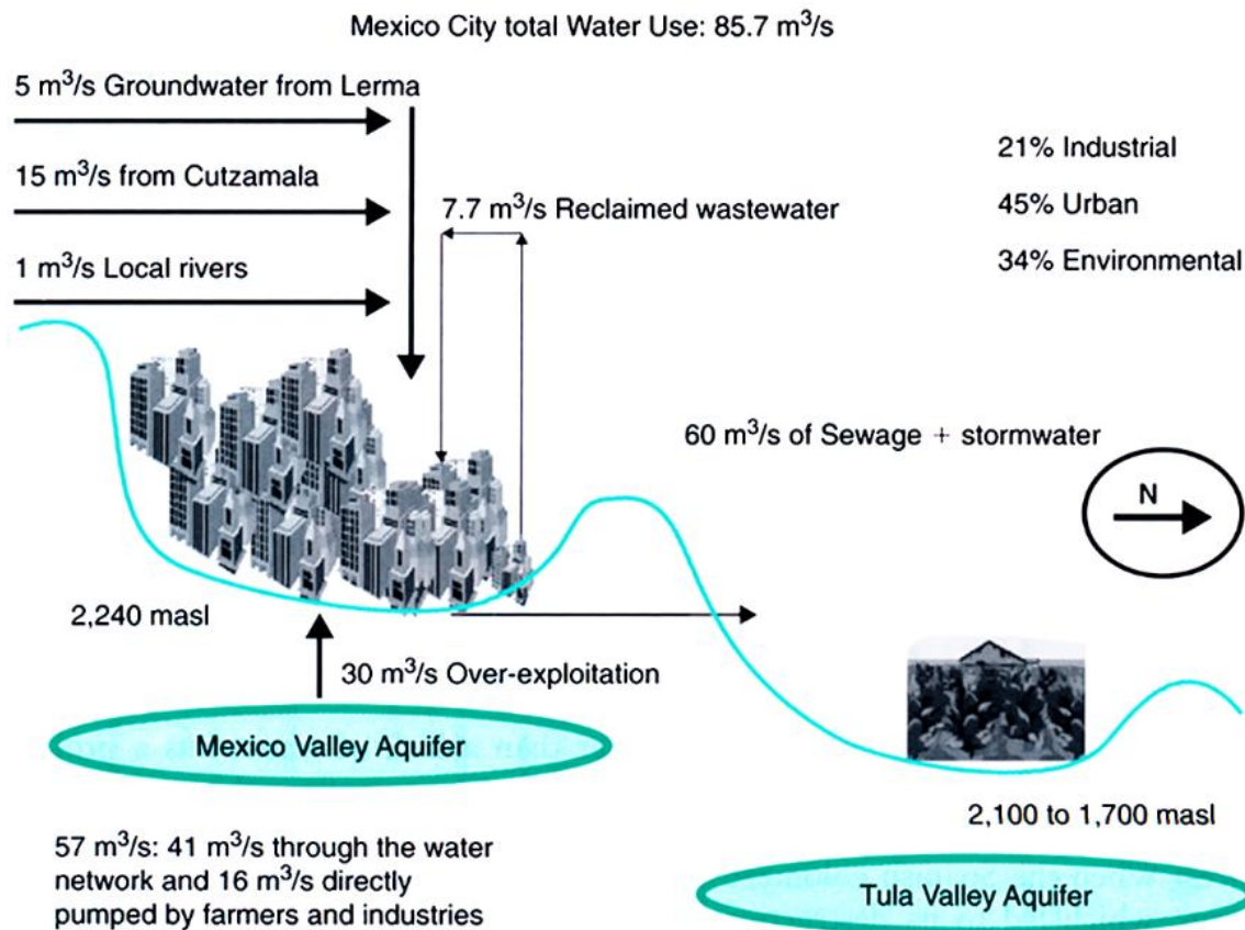
Figure 69 - Water budget for Mexico City during the early part of the twenty-first century (modified after Jiménez, 2009).
