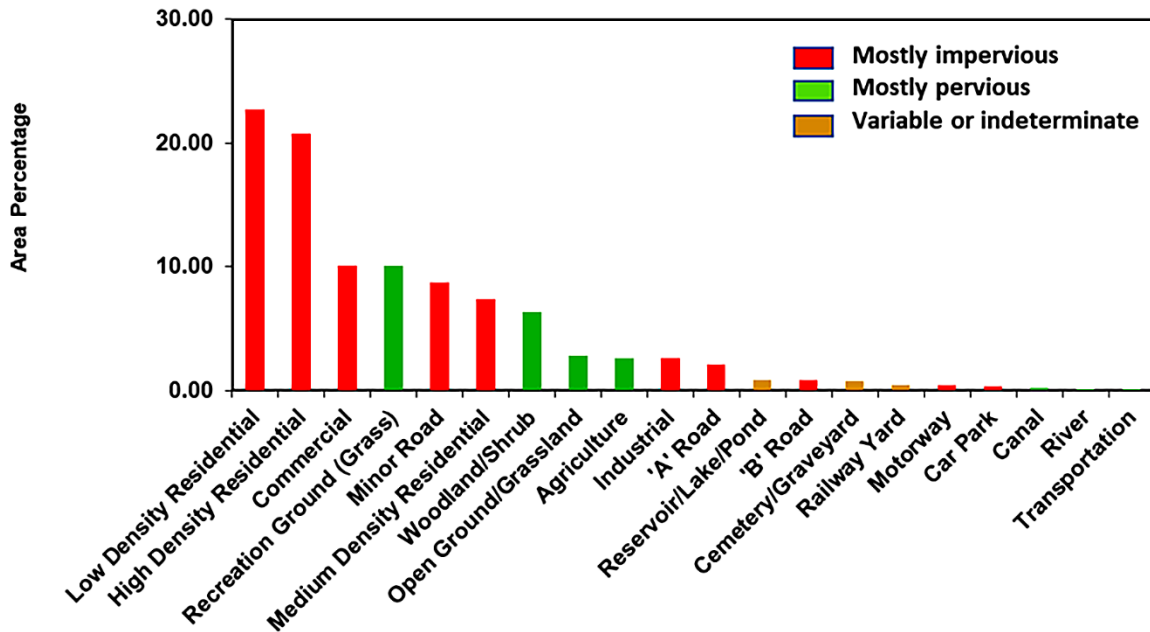
Figure 11 - The relative proportions of land cover in the unconfined portion of the Birmingham urban sandstone aquifer, United Kingdom (modified after Thomas & Tellam, 2006a).
