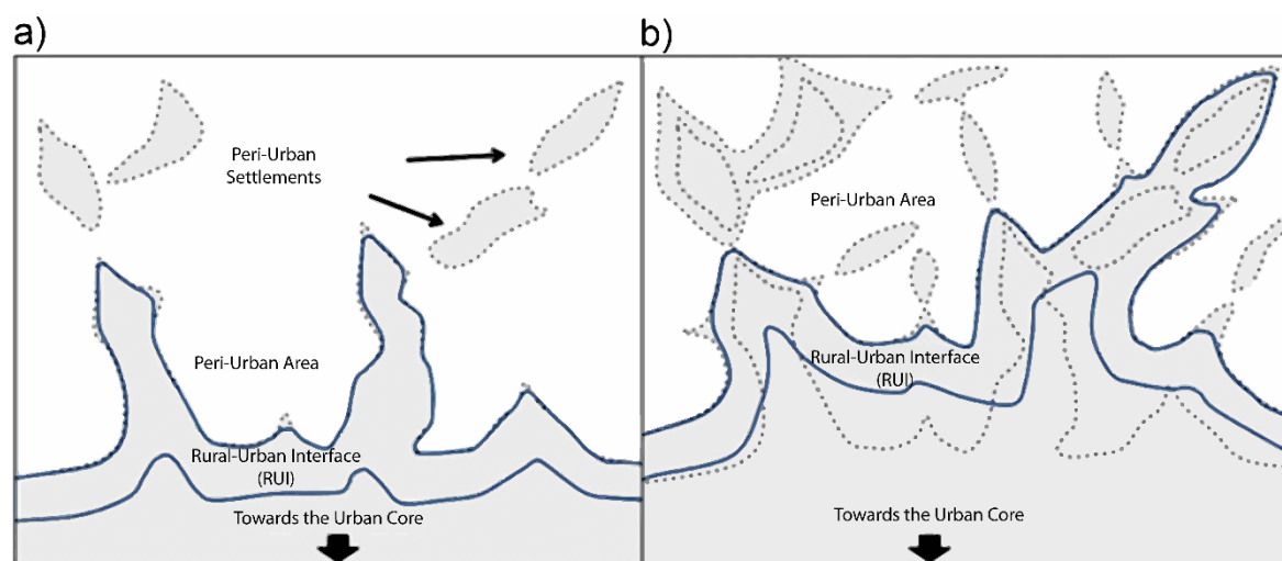
Figure 57 - Two stages of urban expansion: a) and, later, b). In each case, shaded areas are populated. The rural-urban interface (between the two solid lines) and the peri-urban area are shown. It should be noted how peri-urban settlements eventually get absorbed into the urban area and new, peri-urban settlements grow (after Howard, 2012).
