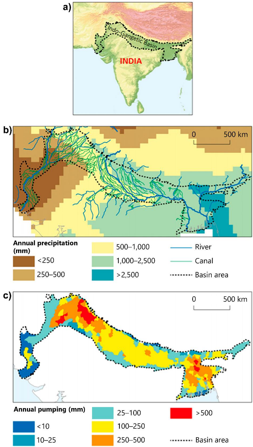
Figure 60 - The location, hydrology, and pumping from the IGB aquifer system: a) Location of the IGB in the Indian subcontinent; b) Mean annual precipitation from 1950 to 2010 and rivers and major canal distribution; c) Estimated mean annual groundwater abstraction in 2010, showing the high groundwater abstraction in northwest India, northern Pakistan, and central and northern Bangladesh (modified after MacDonald et al., 2016).
