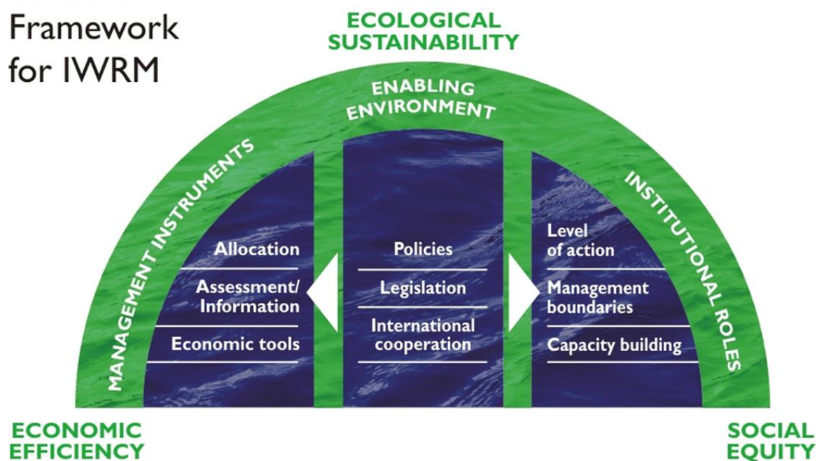
Figure 122 - General framework for Integrated Water Resource Management (JFT Consulting, 2021).
