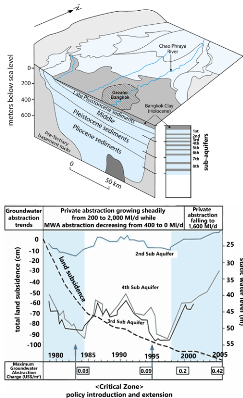
Figure 75 - By the late 1990s, the system was eventually stabilized through science-based groundwater management (Buapeng & Foster, 2008).
