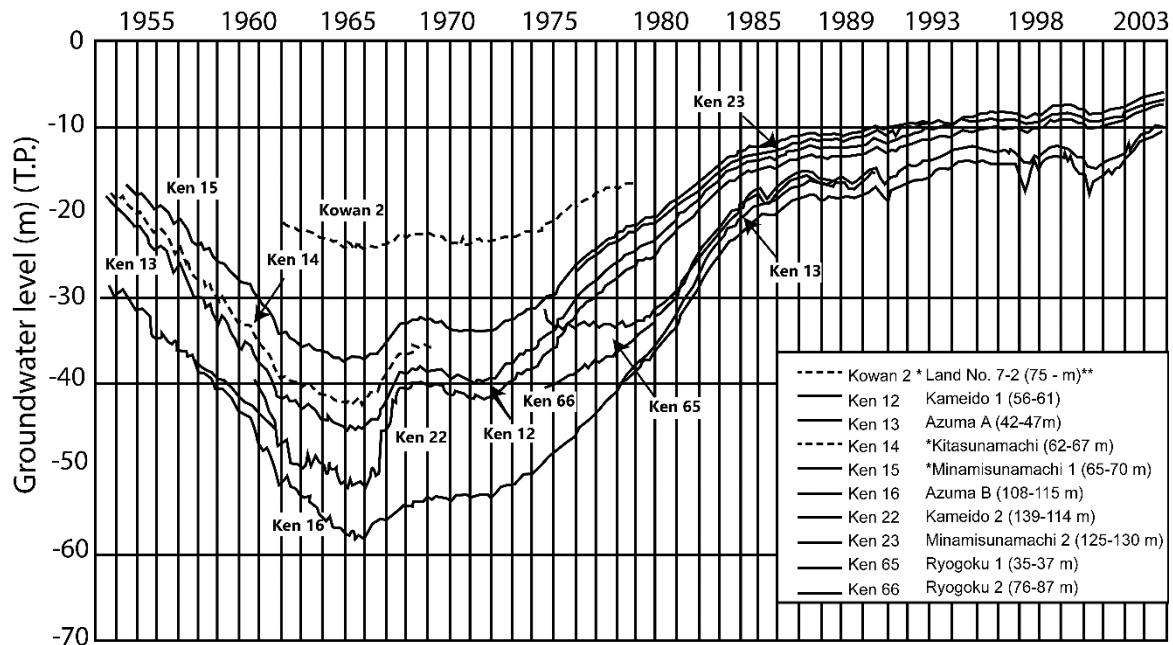
Figure 71 - Variation in groundwater levels in wells in the districts of Koto-ku and Sumida-ku between the early 1950s and 2003. A single asterisk indicates the former site of a well and the double asterisks refer to parentheses which contain values indicating screened intervals (modified after Sato et al., 2006; source: Tokyo Metropolitan Research Institute for Civil Engineering Technology, 2004).
