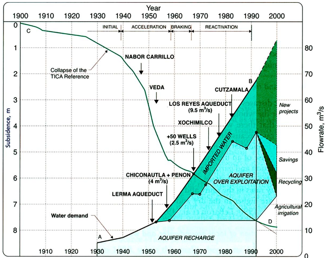
Figure 68 - Mexico City subsidence between 1900 and 2000 in relation to aquifer development. The subsidence problem appears to be under control since pumping rates began to be strictly reduced to avoid over-pumping, alternative water supplies were imported following a socioeconomic analysis, and the city introduced conjunctive management of groundwater resources with surface water. The period from 1990 to 2000 displays projected flow rates for new thrusts related to irrigation, recycling, conservation savings and new imported water projects. For the period 1990 to 2000, the magnitude of recharge was not available when the diagram was created and subsidence is shown as an extended straight line (thin black line) along with the anticipated projection (green line labeled D) suggesting stabilization (modified after Jiménez, 2009; source: Santoyo et al., 2005).
