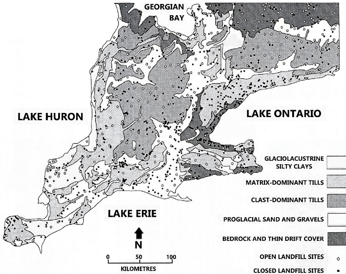
Figure 39 - Location of open (n=311) and closed (n=868) landfill sites in southern Ontario, Canada, in relation to the surficial geology (after Eyles & Boyce, 1997).
