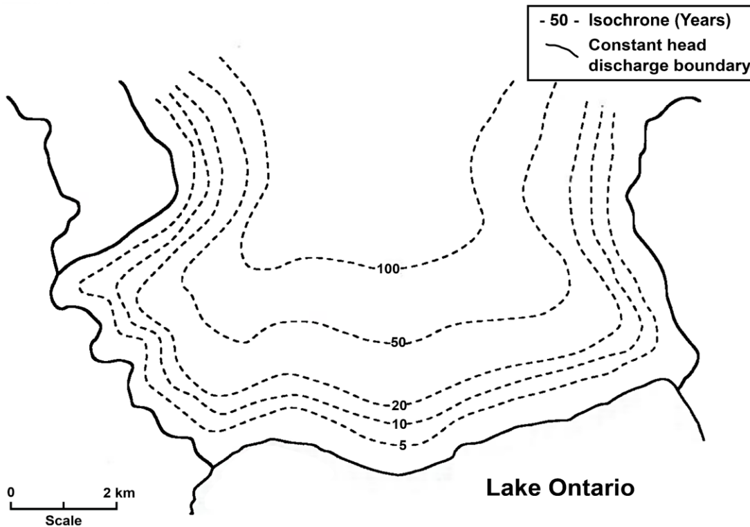
Figure 51 - Contaminant transport isochrones (travel times) shown for the City of Toronto urban core as shown in Figure 48. Travel times assume chemically conservative behavior (retardation factor = 1) (from Howard et al., 1993).
