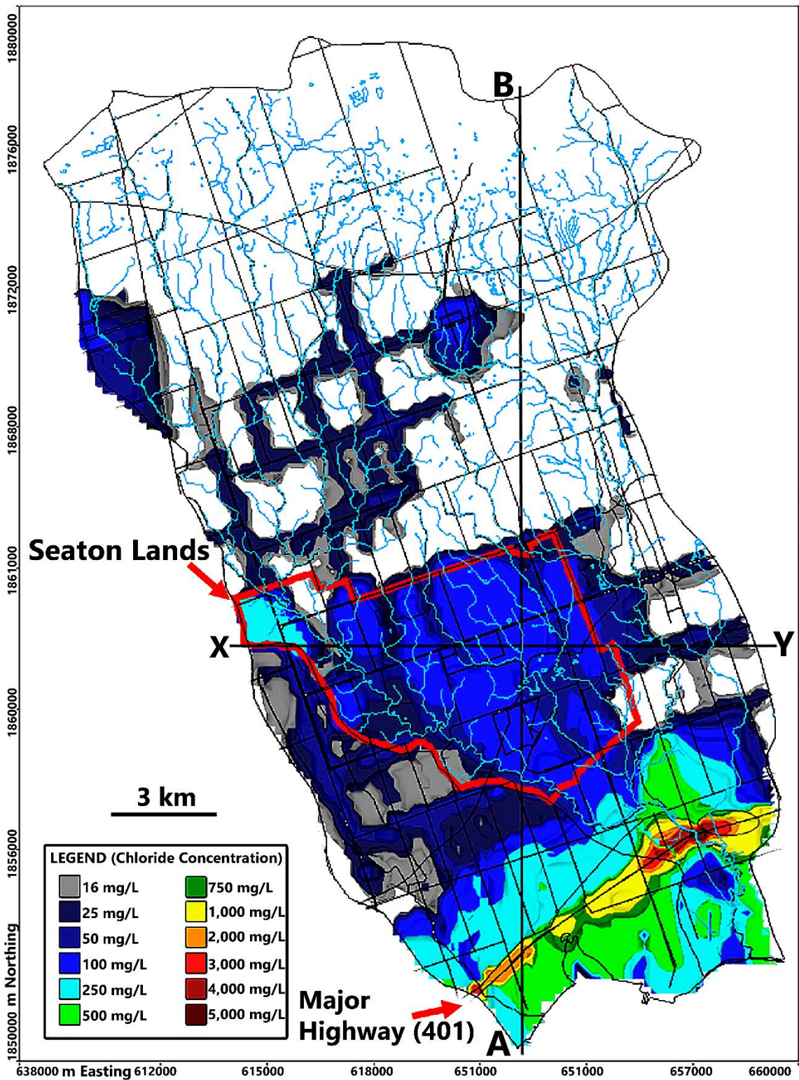
Figure 106 - Predicted long-term, steady-state chloride concentrations in the uppermost aquifer due to road salt application following development of the Seaton Lands study area. The development significantly increases chloride concentrations in the uppermost aquifer (Howard & Maier, 2007).
