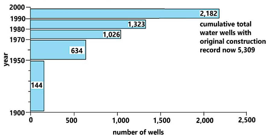
Figure 129 - Attempts to regularize the private use of urban groundwater have been made in places (e.g., Fortaleza in Brazil) where the municipal utility has argued for the levying of a volumetric water charge to reflect mains sewer use by private groundwater abstractors (Modified after Foster et al., 2006).
