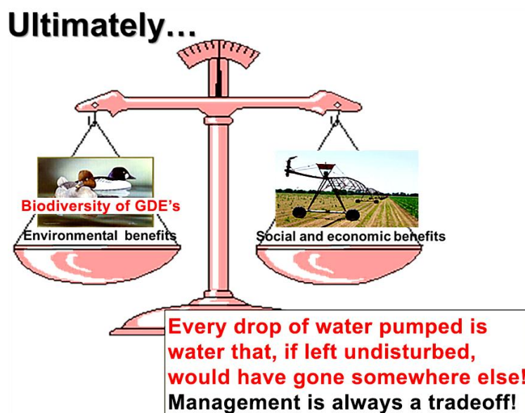
Figure 90 - Aquifer management is always a tradeoff. Decision making needs to balance the social and economic benefits of pumping with the potential environmental benefits of allowing the groundwater to fulfill its normal hydrologic function (from personal files of Ken Howard).
