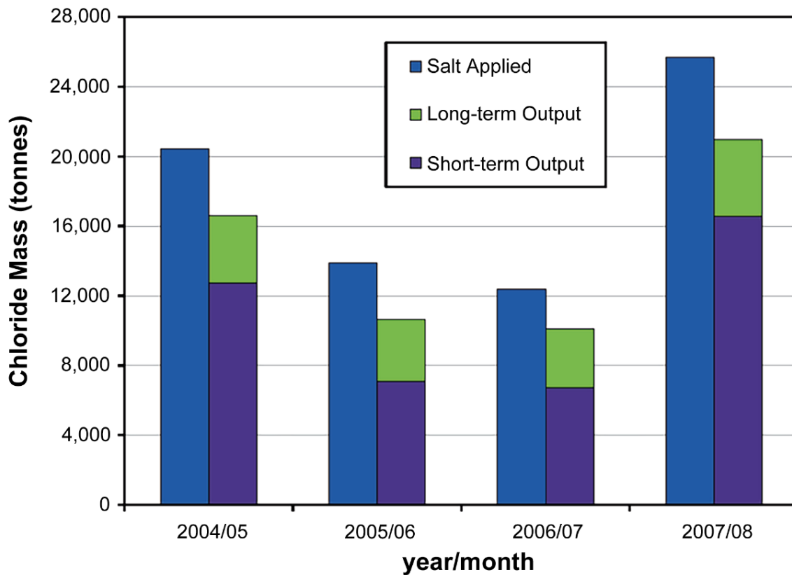
Figure 55 - Annual chloride mass balance for the Highland Creek watershed, Toronto, Canada. Short-term output refers to chloride transported via a combination of surface water runoff (overland flow) and preferential groundwater flow paths associated with urban karst. Approximately 60 percent of the chloride applied to the watershed each salting season gets flushed into Lake Ontario as short-term output, typically within 6 to 12 months of being applied. Long-term output refers to salt that enters the subsurface but does not take advantage of the preferential groundwater flow paths. It enters the stream as baseflow after many decades of travel. For the periods investigated, long-term output represents about 20 percent of the salt applied with the last 20 percent remaining in the groundwater system and increasing concentrations (after Perera et al., 2013).
