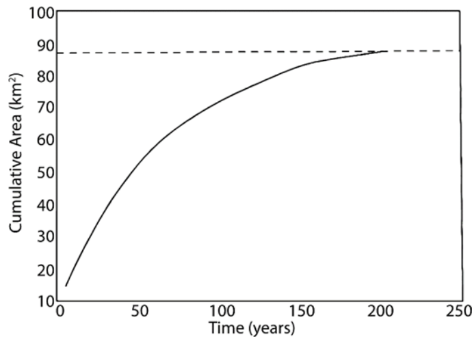
Figure 52 - Cumulative area curve for travel-time isochrones in the case of a chemically conservative contaminant such as chloride. Assuming source input remains unchanged, chemical steady state (input load = output load) is approached after 200 years (from Howard et al., 1993).
