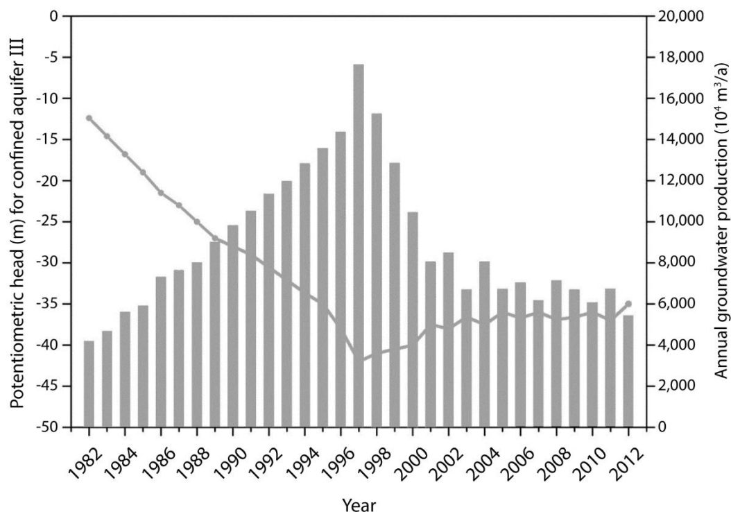
Figure 21 - Annual rate of groundwater abstraction (bars) from confined aquifer III, Nantong, China, between 1982 and 2012 in relation to the potentiometric head (continuous line) in observation well no. 62771502, screened in the same aquifer (Ma et al., 2018). The figure shows how, over a period of just 15 years, a four-fold increase in groundwater production in Nantong led to a 30 m drop in aquifer water level. In the late 1990s, concerns over land subsidence prompted a rapid cutback in production and a steady albeit slow water level recovery. Aquifer modeling is now being used to investigate options for distributing pumping regionally and across all aquifers to optimize the yield of the aquifer system (Ma et al., 2018).
