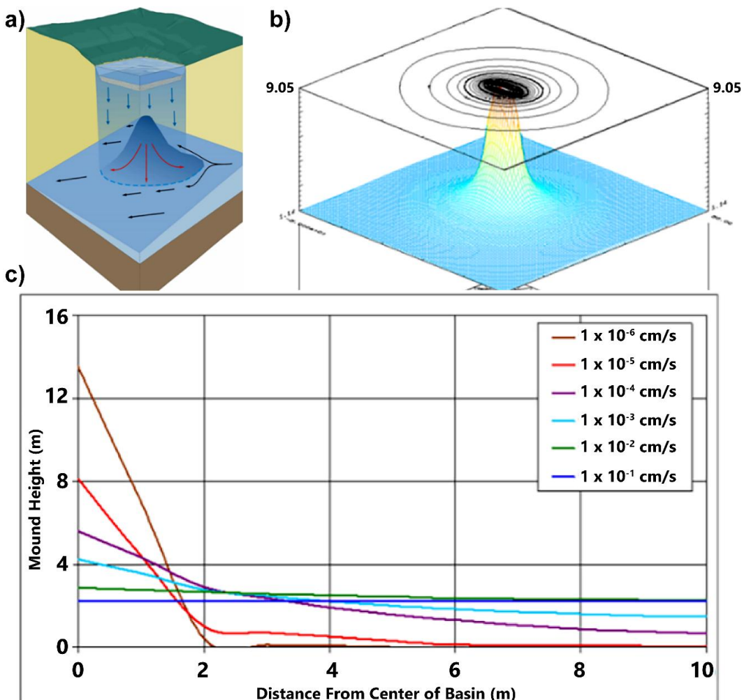
Figure 84 - The height of the recharge mound that develops beneath the basin is a limiting feature. a) Schematic of flow through a recharge mound and into the underlying aquifer. b) Three-dimensional rendering of the mound surface with water elevation projected to the surface as contour lines of equal head. c) Permeable sediments are required to ensure the recharge mound is not so high that it limits infiltration rate (Howard et al, 2007).
