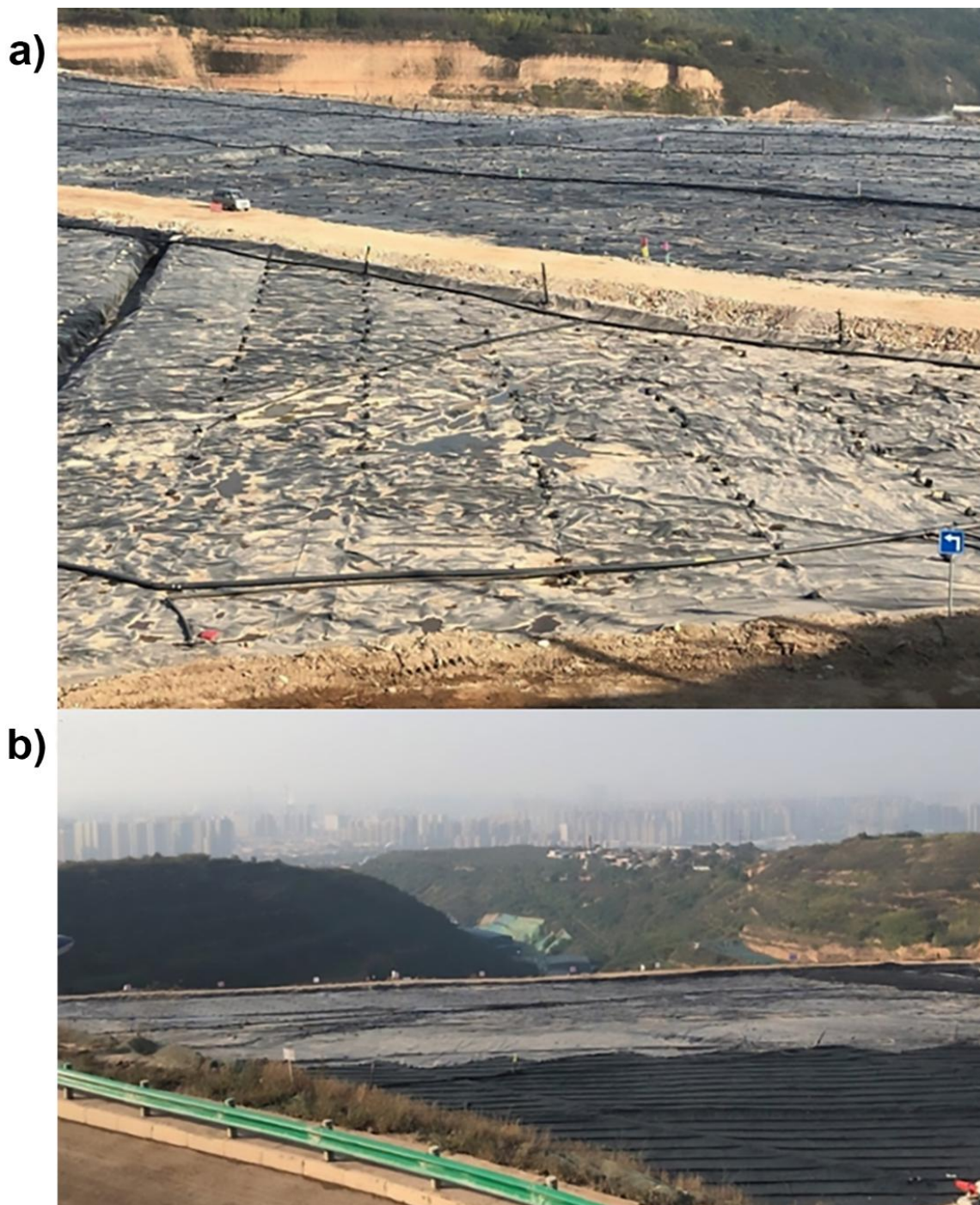
Figure 40 - a) The Jiangcungou landfill in Xi'an, China, lies at high elevation and fills a deep, narrow valley on the outskirts of the city. The landfill is partially engineered and covered b) to reduce leachate generation; however, serious concerns have been expressed over the potential for subsurface contaminant plume migration. The landfill is now closed (photography by Ken Howard).
