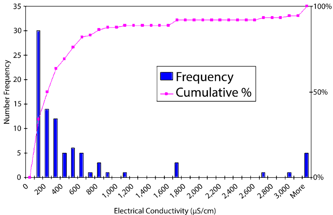
Figure 48 - The electrical conductivity of road drain gully pot waters from the campus of the University of Birmingham, United Kingdom. Samples were collected mainly in winter, spring, and autumn. Maximum conductivity recorded was found to exceed 100,000 \mu\text{S}/\text{cm} (characteristic of brine) (from Harris, 2007).
