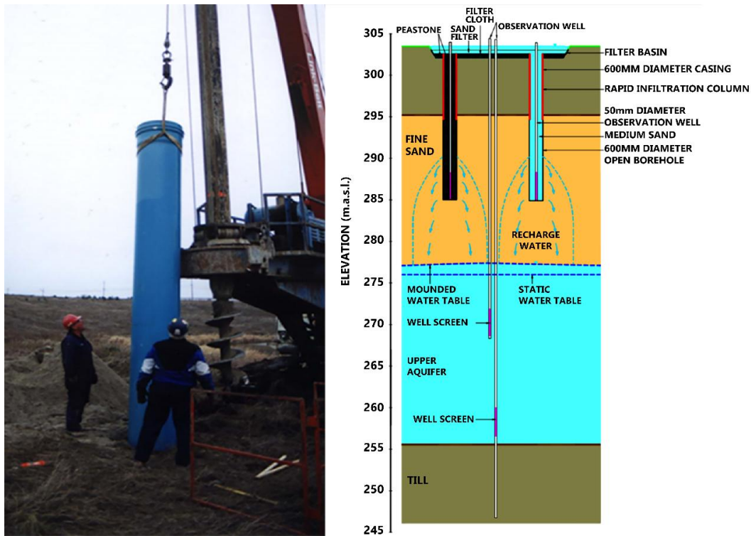
Figure 85 - Rapid infiltration columns (RICs) can be used to allow infiltrated water to bypass low permeability materials such as glacial tills (photography by Ken Howard).
