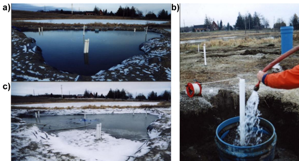
Figure 86 - Rapid infiltration columns (RICs) work well even during winter when ice develops across the basin. a) Unfrozen recharge pond b) water is being added to infiltration column to test its ability to accommodate recharge c) Frozen recharge pond (photography by Ken Howard).
