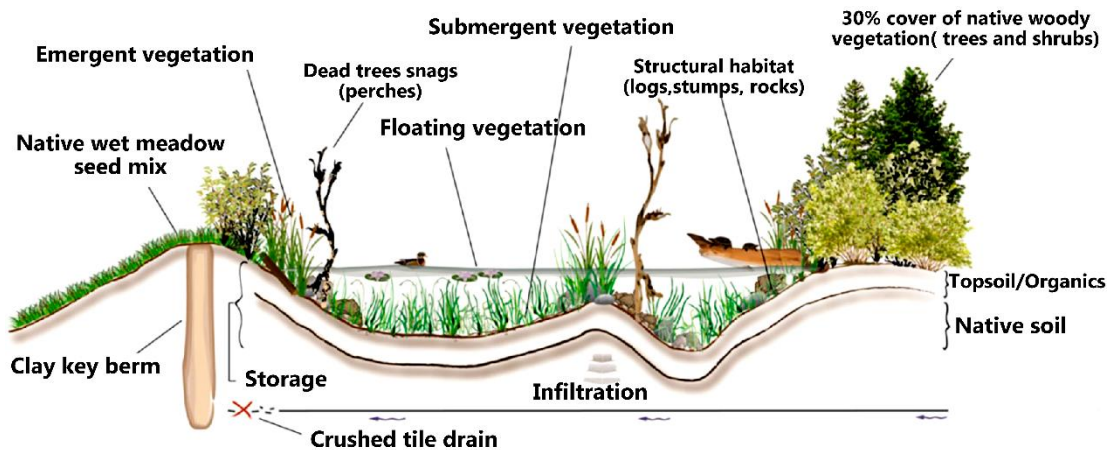
Figure 47 - Design example for a constructed wetland (diagram credit: Toronto & Region Conservation Authority).
