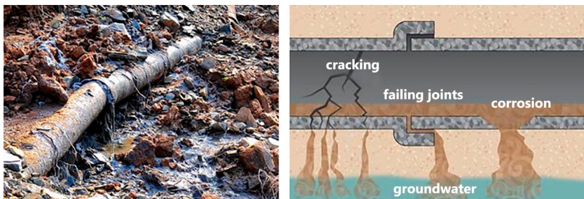
Figure 35 - A 2017 study undertaken by staff at the City of Albuquerque, Texas, USA, estimated that the sewage collection system lost 11 percent of wastewater due to exfiltration (photography from personal collection of Ken Howard; diagram from Bhatia, 2017).
