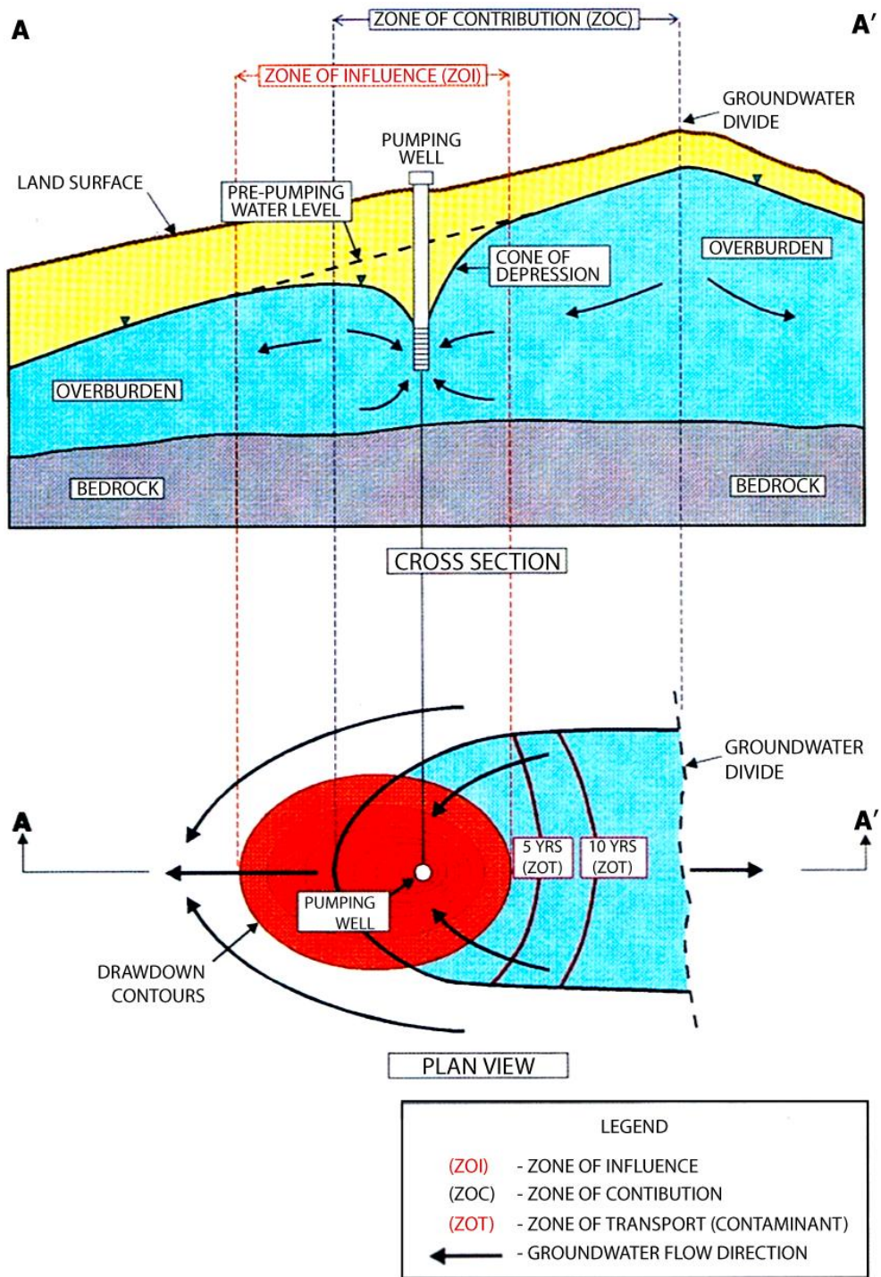
Figure 100 - Conceptual representation of wellhead protection areas and terminology for an aquifer with a sloping water table adjacent to a groundwater divide (modified after Livingstone et al., 1997).
