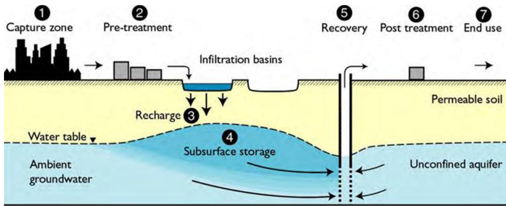
Figure 88 - Schematic showing how wastewater captured from a city can be pre-treated and infiltrated for subsequent recovery and post treatment prior to its eventual use (from Natural Resource Management Ministerial Council, Environment Protection and Heritage Council, & National Health and Medical Research Council, 2009).
