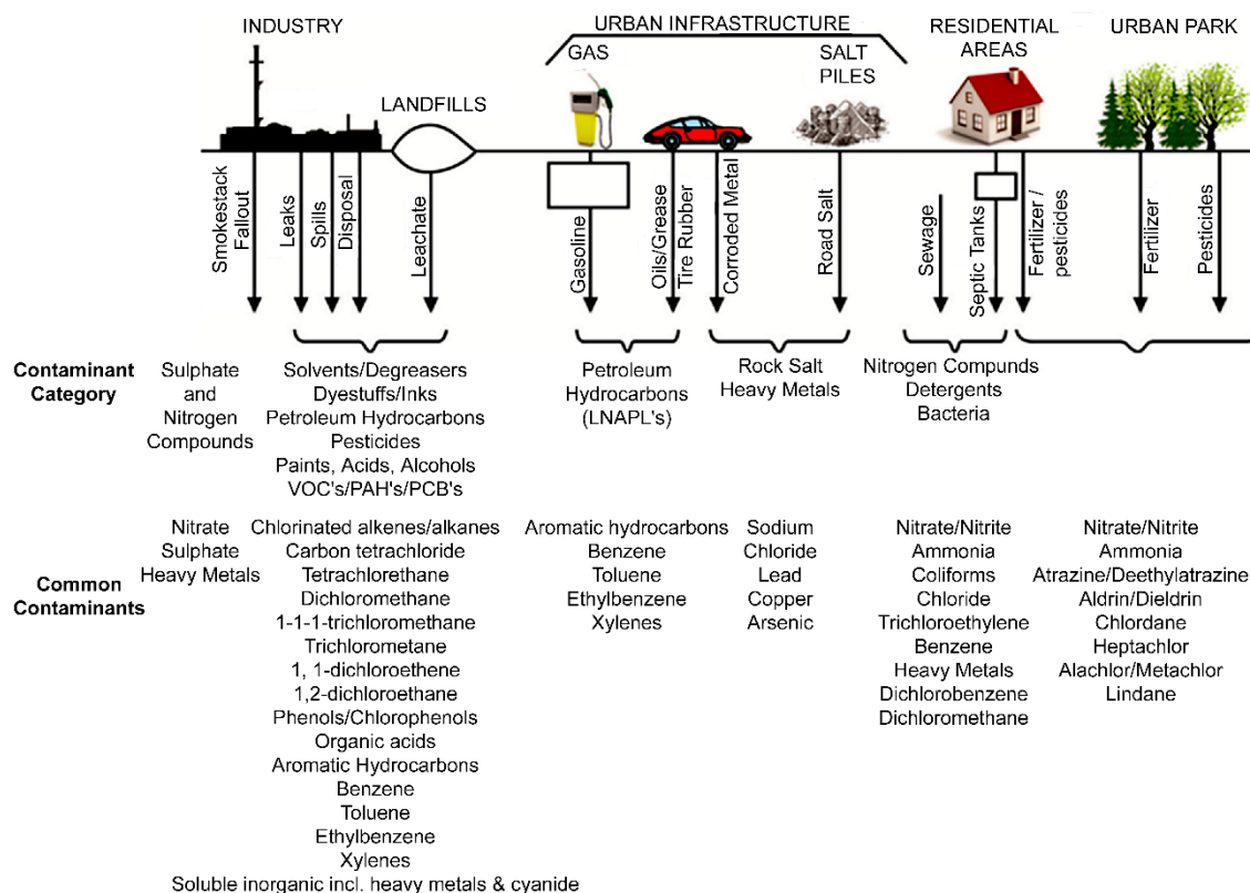
Figure 30 - Common sources of urban groundwater contamination (from Warner et al., 2016; modified after Howard, 1997).
