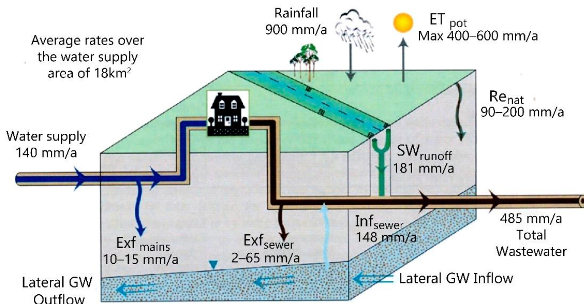
Figure 36 - Water balance studies in the City of Rastatt, Germany, where natural recharge is in the range 90 to 200 mm/a, suggest that sewage exfiltration may contribute an additional 2 to 65 mm/a. ET is evapotranspiration; Inf and Exf are infiltration and exfiltration, respectively; Re is recharge; GW is groundwater (modified after Wolf et al., 2006).
