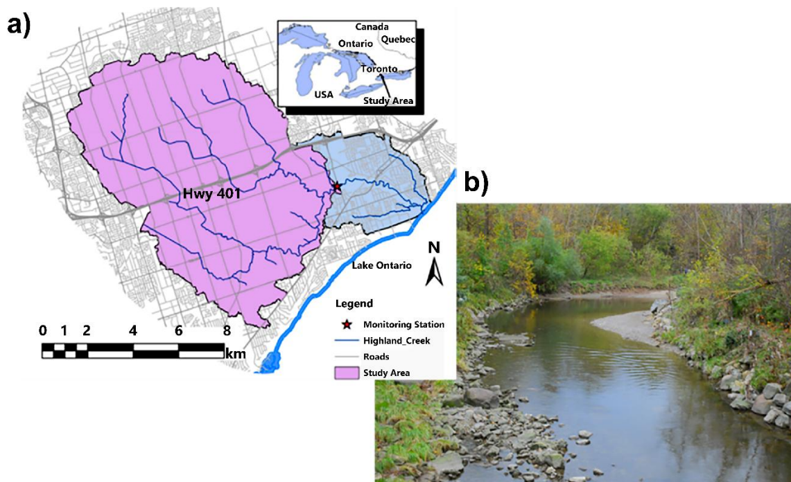
Figure 43 - Highland Creek catchment in eastern Toronto, Canada, showing the location of the gauging station where stream water quality and flow was observed (a) from Perera et al, 2013; b) photography by Ken Howard).
