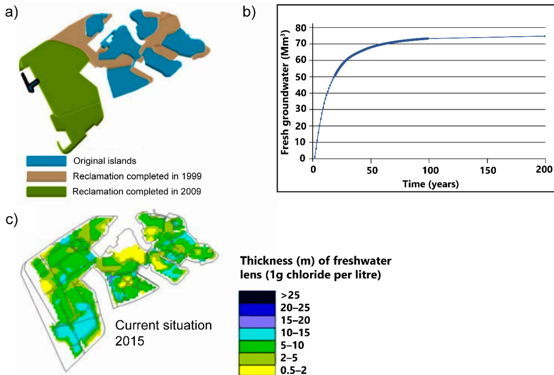
Figure 82 - a) Development of Jurong Island over time; b) Full development of the fresh groundwater lens (1 gm/L chloride) may take well over 50 years (initial groundwater salinity was 18 gm/L); c) Thickness of the freshwater lens on the island in 2015 (locally 10 to 15 m; figure modified after Saha et al., 2016).
