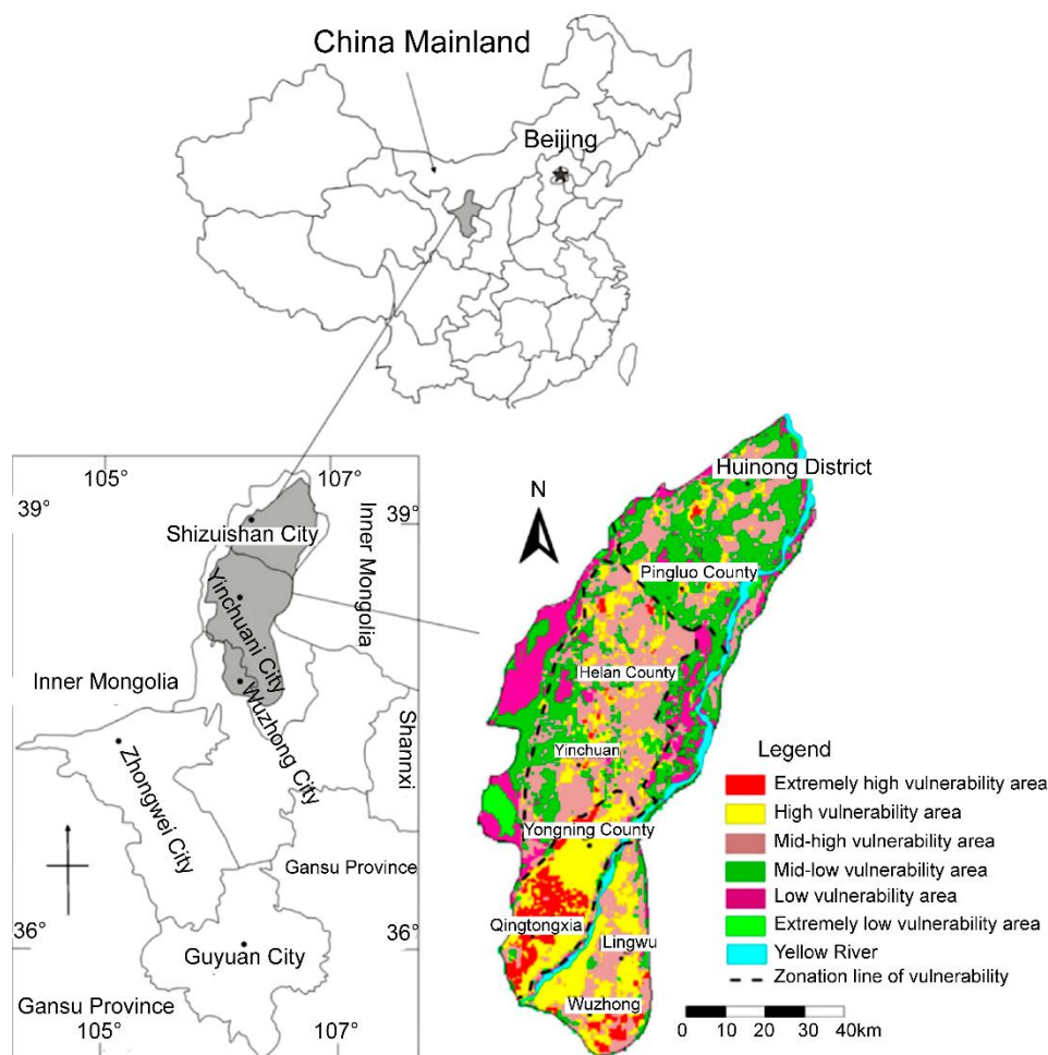
Figure 98 - Intrinsic aquifer vulnerability rankings for aquifers underlying the heavily populated Yinchuan Plain using OREADIC, an adaptation of DRASTIC (modified after Qian et al., 2011).
