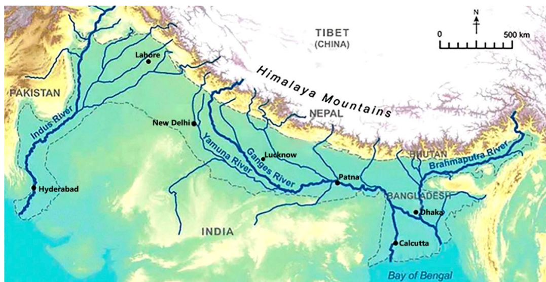
Figure 59 - Location map of the Indo-Gangetic Basin (IGB) alluvial aquifer, shown within the dashed line and with topography as background. The cities of Lucknow and New Delhi are shown (modified after Bonsor et al., 2017)
