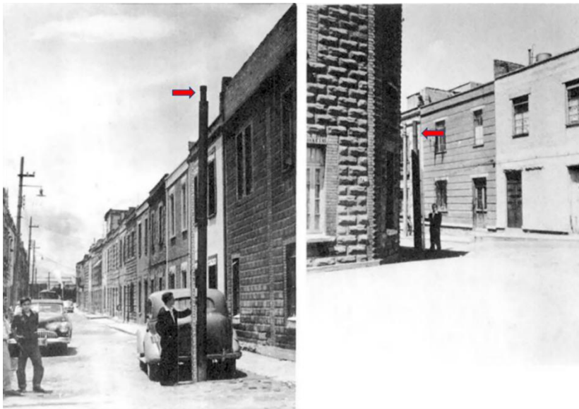
Figure 67 - Protrusion of well casings (arrowed) in the northern part of Mexico City. The wells were drilled around 1923, probably 100 m deep and the photos were taken some 30 years later in 1954. The casing to the left protrudes 5.45 m; the casing to the right protrudes 4.50 m. (from Poland & Davis, 1969) (photography by Ing R. Marsal).
