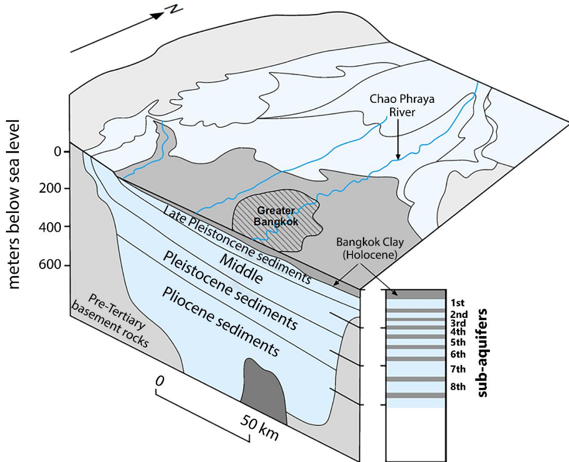
Figure 72 - Hydrogeological block diagram showing structure of the Middle and Lower Chao Phraya alluvial aquifer system in relation to Greater Bangkok (from Buapeng & Foster, 2008).
