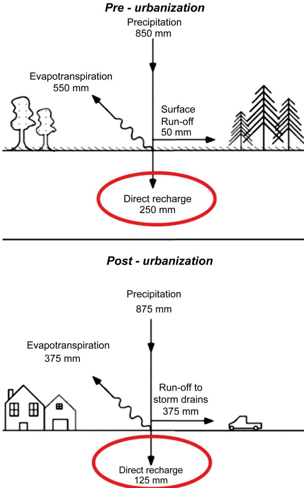
Figure 12 - Reduction in direct recharge in a typical urban area under temperate climate conditions where a small increase in precipitation due to the urban heat island effect is offset by increased runoff resulting in less recharge (after Howard, 1997).
