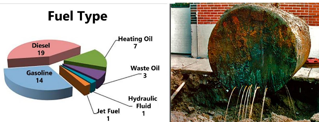
Figure 34 - In 2017, the Montana Department of Environmental Quality (USA) reported a 10-year high of 45 confirmed petroleum releases from underground storage tanks, with the product types displayed in the pie chart. Forty percent of the cases were associated with corrosion and equipment failure; over 50 percent were due to negligence (photography by Montana Department of Environmental Quality).
