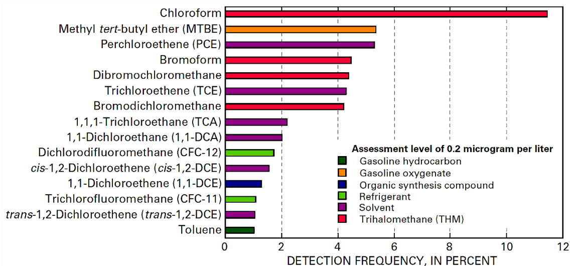
Figure 32 - Detection frequencies in samples from the public supply wells at a detection level of 0.2 µg/L. Trihalomethanes, solvents, and the gasoline oxygenate MTBE were among the 15 most frequently detected VOCs (after Zogorski et al., 2006).
