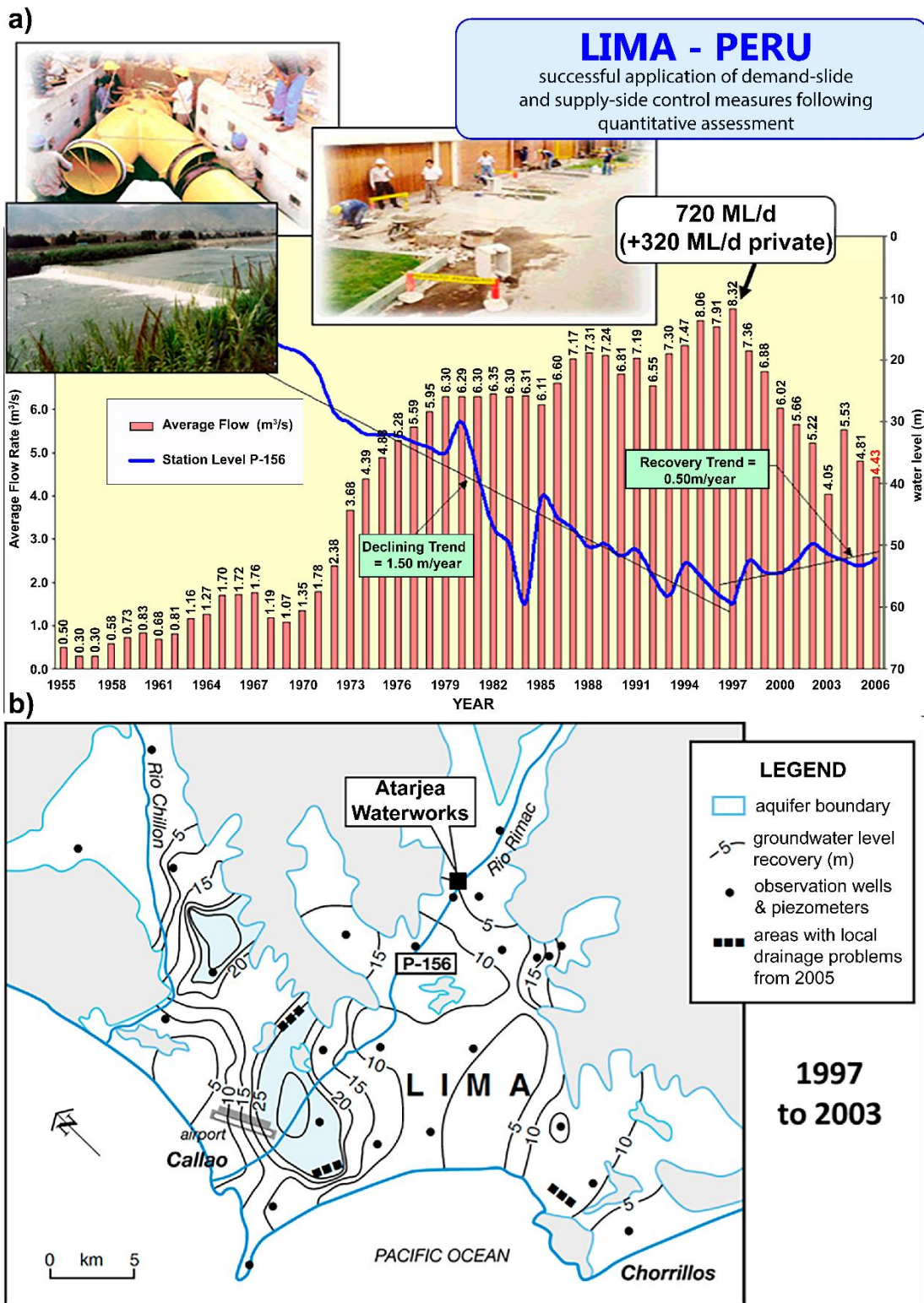
Figure 128 - In Lima, Peru, successful application of demand-side and supply-side control measures (supported by conjunctive use of ground and surface water) led to a) stabilization and steady recovery of groundwater levels, b) as mapped in the Lima area with 5 km/≈3 miles (modified after Foster et al., 2010d).
