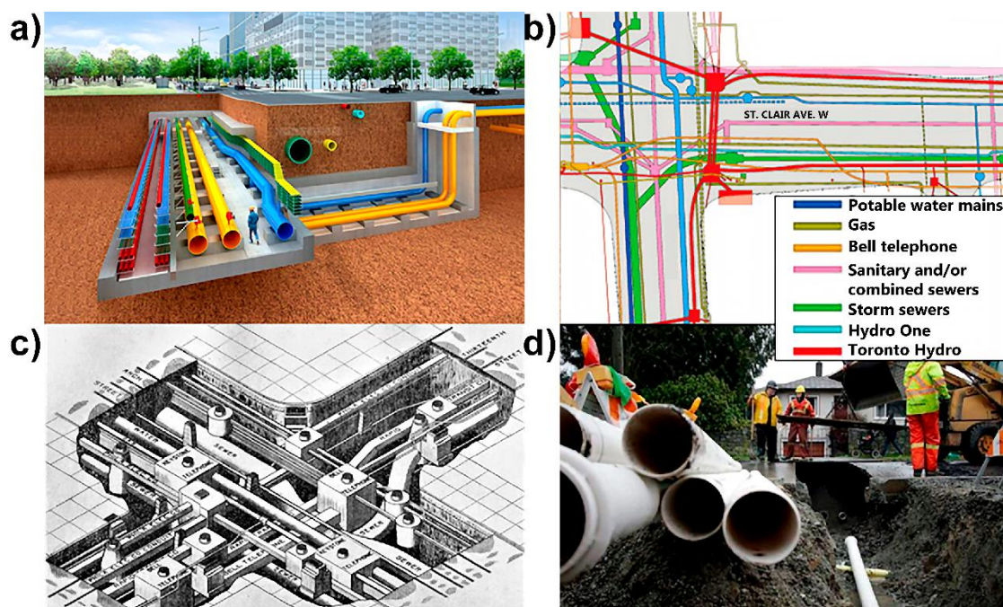
Figure 27 - Beneath urban areas, a complex network of drains, pipes, and tunnels create urban karst or epi-karst, a shallow artificial aquifer that exerts a major—yet often unpredictable—influence on aquifer recharge, groundwater flow, and contaminant transport. The term urban karst has been used for many years (Sharp et al., 2001; Krothe, 2002; Krothe et al., 2002; Sharp et al., 2003; Garcia-Fresca, 2007) to describe the secondary permeability and porosity that develops in association with subsurface construction activities. While trenches and drains lined with permeable material are usually the primary contributors, the term is often used to include any enhancement of permeability and porosity that is created by urbanization, either directly or indirectly (photographs from personal collection of Ken Howard).
