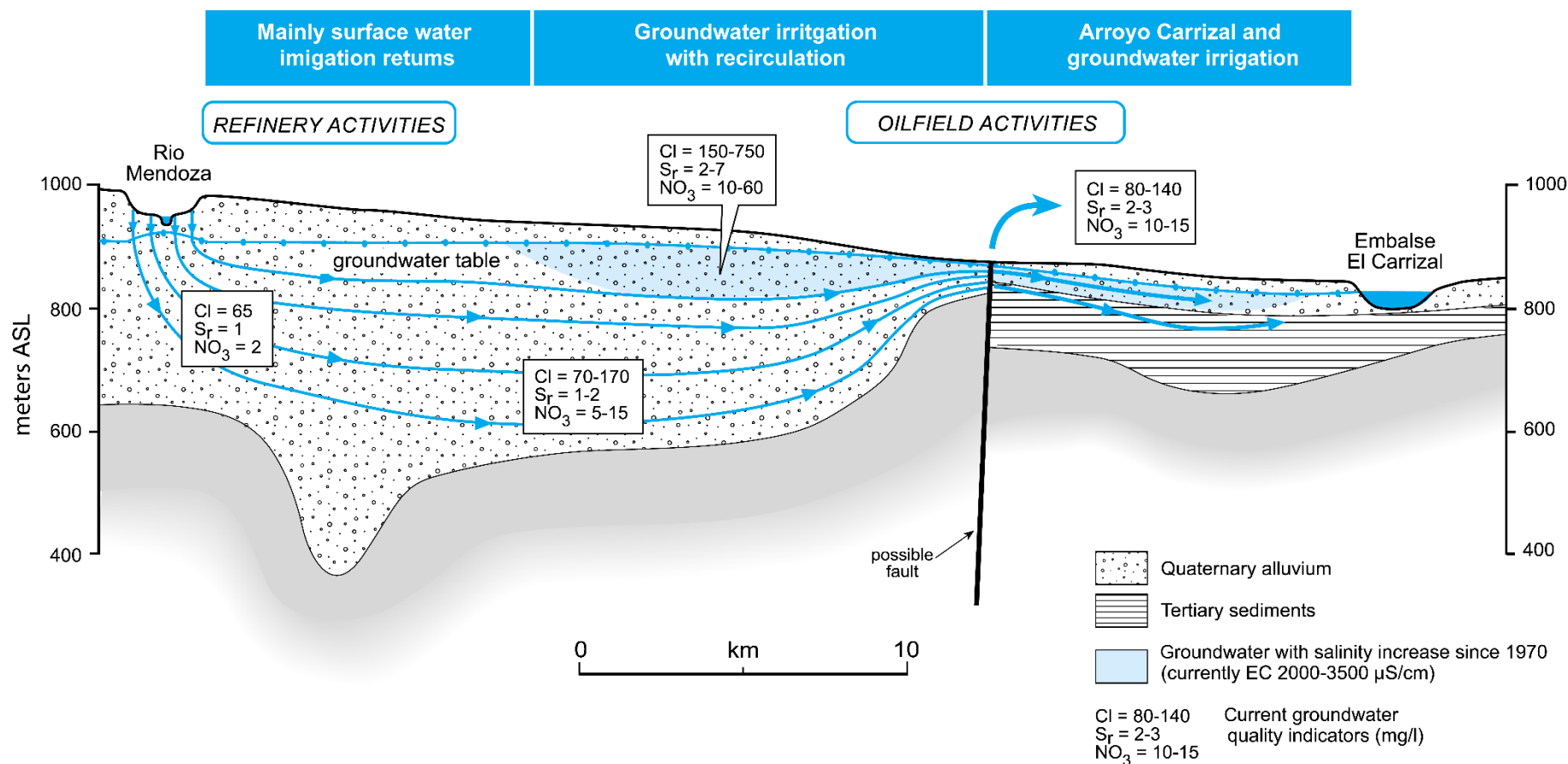
Figure Box 2-1 - Hydrogeological profile along the flow direction of the Carrizal aquifer system (from Foster & Garduño, 2006). The General Department for Irrigation [Departamento General de Irrigación; DGI] is the autonomous water resource authority responsible for water management in the entire province, down to the primary canals and the delivery of water to the Water Users' Associations (WUAs). Groundwater abstraction is the main source of water for irrigation outside the command network of main canals and is used to supplement surface water during times of critical plant demand and in years of low flow.
