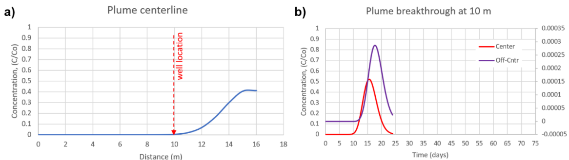
Figure Exercise 3-2 – a) Concentration of tracer along the centerline of the plume at each instant in time which is a 'profile of the pulse' with the red dashed line showing the location of the well. b) Breakthrough curves of concentration in each of two wells located 10 m from the injection well.
