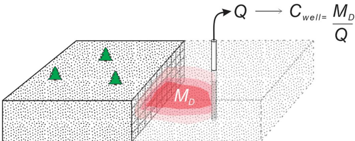
Figure 25 - A plume is captured by a water-supply well. If the mass discharge of a contaminant in the aquifer is known, the concentration that will appear in the well, C_{well} , can be anticipated for any rate of pumping, Q , that captures all of the plume. The simple relationship shows that C_{well} is proportional to M_D , e.g., doubling M_D will double C_{well} .
