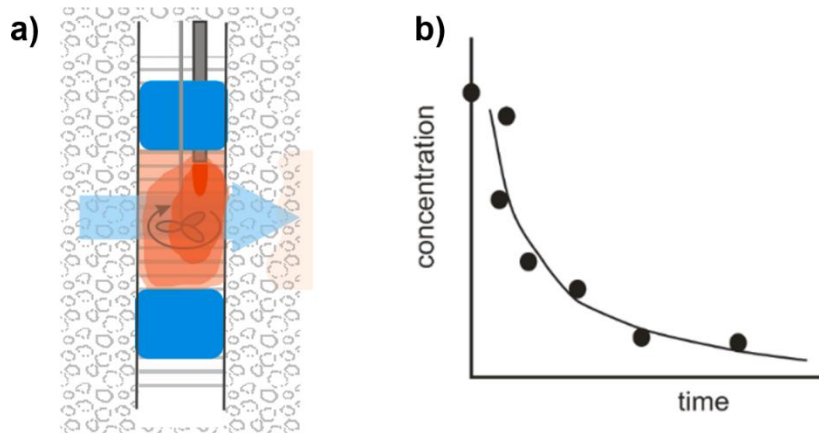
Figure 9 - a) Schematic of the borehole dilution method. Packers (blue) isolate a section of the well while a tracer (red) is mixed (black arrow) with groundwater in the test interval. b) If mixing is continuously maintained, the tracer concentration in the test interval declines exponentially as groundwater passes through the well (see graph).
