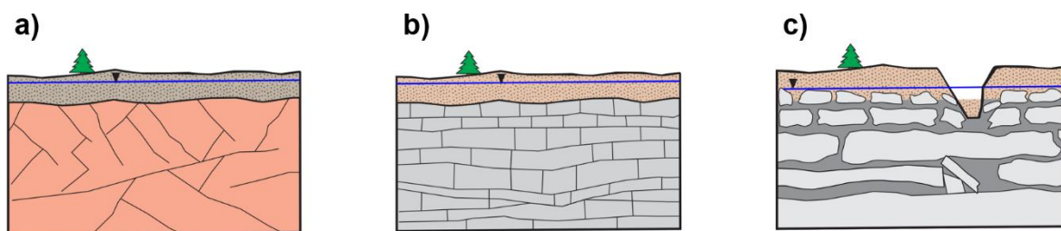
Figure 26 - Conceptual diagrams of three types of fractured rock. a) fractured crystalline rock with relatively low aperture openings associated with faulting, jointing, and fracturing from regional or local tectonic activity, or other geologic processes. b) sedimentary rock with openings associated with bedding planes or fracturing due to local or regional tectonic activity or other geologic processes. c) highly weathered rock such as karst with openings ranging from micron sized apertures to cave conduits, and collapse features like sinkholes that allow surface water to rapidly enter the subsurface.
