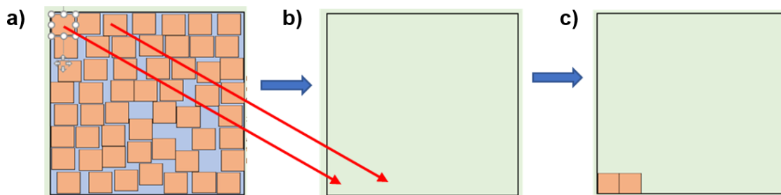
Figure Exercise 1-1 - a) Imperfectly packed grains of an aquifer sample are to be moved into panel b) the total space of the sample so that in c) they are stacked in a closely packed arrangement.
