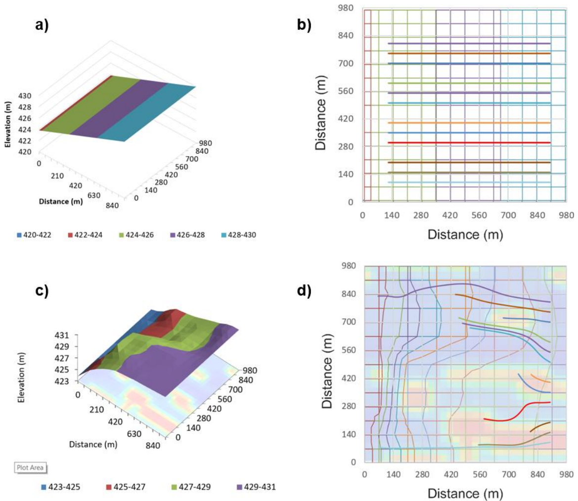
Figure 19 - a) Equipotential surface (with water level contours) for a hypothetical homogeneous flow system with hydraulic conductivity of 2.5 m/d and an overall gradient across the domain of 0.001 causing flow from right to left. b) Traces of 12 particles transported for 40 years (porosity assumed to be 0.3). Note all particles travel the same distance in the same direction, indicating a plume in this setting would remain intact and undergo minimal mixing from causes related to groundwater velocity. c) Same flow system as (a) showing the water level surface in three dimensions for the case where the aquifer is heterogeneous with lenses of K ranging from 0.25 (blue) to 25 m/d (red) (shown on the x-y plane). d) The traces of the same 12 particles from (b) released into the heterogeneous flow system shown in (c) for 40 years. Note the variation in particle pathways suggesting considerable plume distortion and splitting, enhancing the conditions that promote mixing at the molecular scale. This effect is solely due to variations in groundwater velocity.
