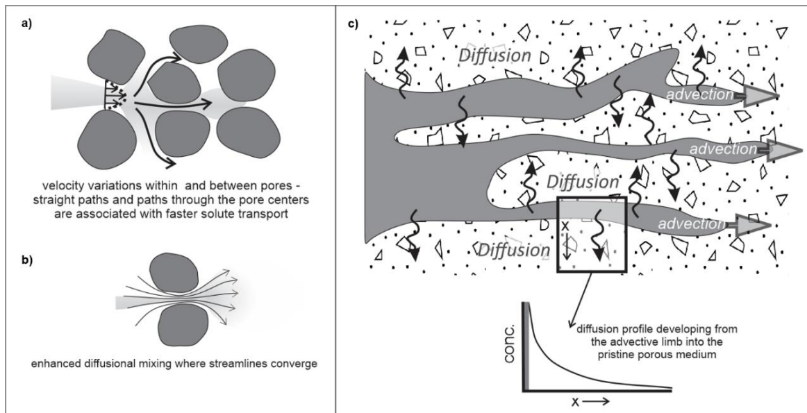
Figure 20 - Historically, dispersion has been visualized as the result of the processes illustrated above. These processes do not directly cause molecular scale mixing, but they can promote it by creating conditions favorable for diffusion. a) Velocity variations may occur within pores, or between pores resulting in enhanced pollutant concentration gradients (i.e., the difference of concentrations at two points divided by the distance between the points, \Delta C/\Delta x ) in directions transverse to flow. These gradients drive mixing by diffusion, which can occur over short time scales at the pore scale. b) In addition, the compression of streamlines within some pores increase the transverse concentration gradients by decreasing the magnitude of the \Delta x in the \Delta C/\Delta x term. c) Variations in velocity at larger scales can also create zones with high concentration gradients. In such zones, diffusion occurs at the maximum rates for those scales, and mixing is promoted. Note: the diffusion profile shown is provided to illustrate the tendency for pollutant mass to mix with surrounding groundwater by diffusion. A fully developed diffusion profile such as the one shown would be repeatedly disrupted in a transient flow system, or as a plume evolved, and never be achieved. Velocity variations at the pore scale are important over centimeter lengths or less. Velocity variations at the centimeter scale or higher may be of practical concern for characterization and remedial design purposes.
