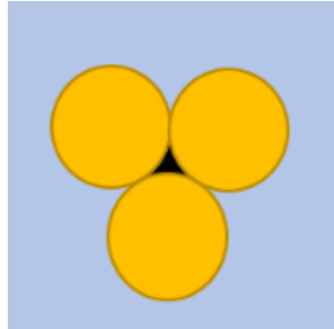
Figure Exercise 1-2 - Example of coloring in a closed pore.
