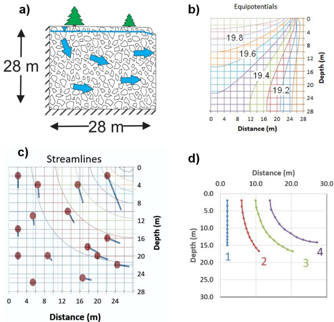
Figure 21 - a) A Cross-section of a simple, homogeneous flow system with a flow divide (no water crosses a divide) on the left and an impermeable base layer. Water recharges from the surface and exits the system at the right boundary. b) Contoured water levels (equipotential lines as elevations in meters) in the aquifer; closer spacing of the lines indicates faster flow. c) Streamlines showing the paths of groundwater flow, and points (red dots) with velocity vectors (blue lines) showing direction of flow and scaled so lines are proportional to the water speed. d) Path lines of four parcels of water originating from different locations in the flow system and traveling for the same period of time. Note that because of its location in the flow system, parcel 4 travels a greater overall distance in the same period of time than parcel 1 — this is particularly evident in terms of the horizontal distances travelled.
