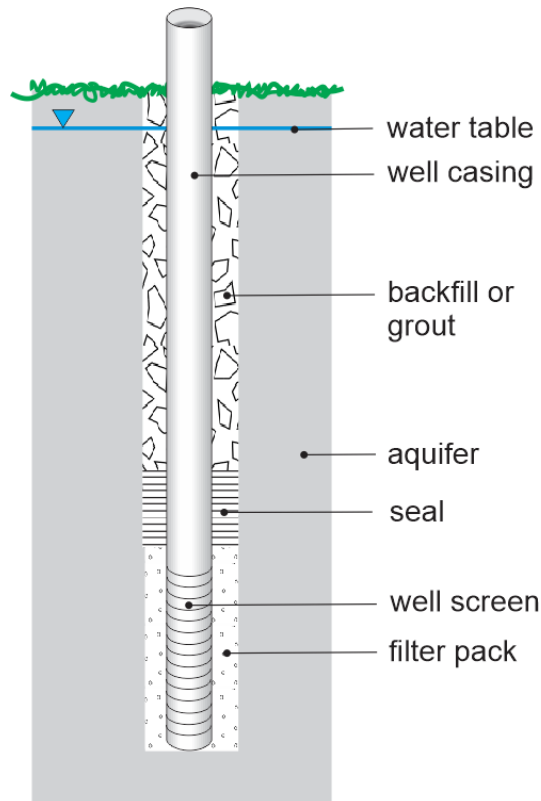
Figure 5 - Schematic of a typical monitoring well (Bedient et al., 1994).
