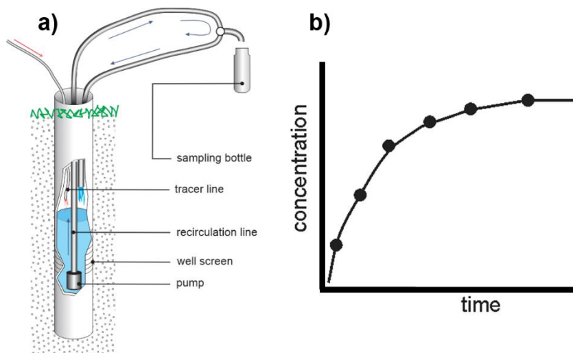
Figure 10 - a) Schematic of the finite volume point dilution technique. b) If mixing and tracer injection are continuous, the tracer concentration rises to a plateau over time.
