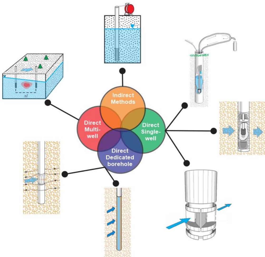
Figure 1 - Contextual diagram showing selected alternative methods for determining groundwater velocity and their general classifications as direct or indirect methods. All are discussed in detail in the following sections of this book. Clockwise from top: Darcy’s Law method, point dilution methods, heat pulse flowmeter method, IWPVP, ISPFs, PVP, and multi-well tracer tests.
