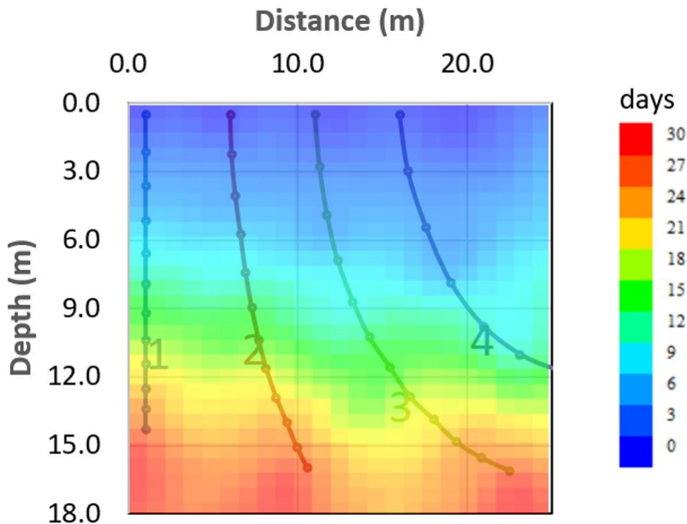
Figure 22 - Cross-sectional view of part of a 30 m by 30 m hypothetical aquifer with 30-day particle tracks and colored isochrons displayed. The calculations performed for this image are approximate, based on the four particles shown and six different times (5, 10, 20, 25, and 30 days), but the near horizontal layering of groundwater ages (or residence times) is also observed in more sophisticated models.
