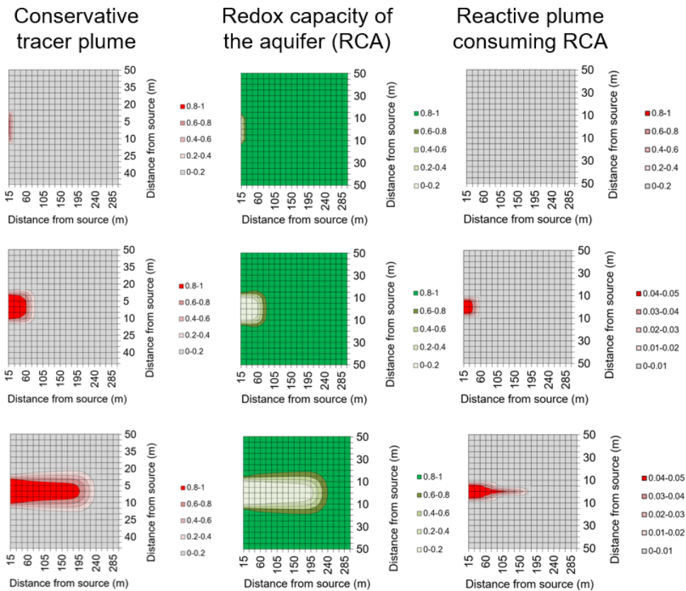
Figure 17 - Progression of contaminant plumes (in plan-view with time advancing down the table) behaving conservatively (left) and susceptible to transformation by oxidation or reduction in an aquifer with a redox capacity (right). The plume growth is retarded by the mass loss due to reaction, and the aquifer redox capacity consumed progressively from left to right over time (center).
