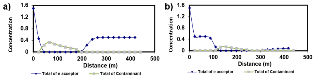
Figure 16 - Two cases of a contaminant reacting with an electron acceptor in a flow system. In both cases the electron acceptor is present in the background water at a concentration of 0.5 \text{ M/L}^3 and has been injected at the source at 1 \text{ M/L}^3 for one year. The plumes are modeled in three dimensions. The contaminant is introduced at 1 \text{ M/L}^3 and has been released for 15 years. a) Plume center line profiles for an oxidizable contaminant and an electron acceptor in an aquifer with a v of 0.1 \text{ m/day} . b) The same plume center line with a v of 0.3 \text{ m/day} . Reactions between the contaminant and the electron acceptor are assumed to be instantaneous. The electron acceptor was assumed to move in the aquifer without retardation, and the contaminant was assumed to migrate with a retardation factor of 2.5, typical of simple hydrocarbons.
