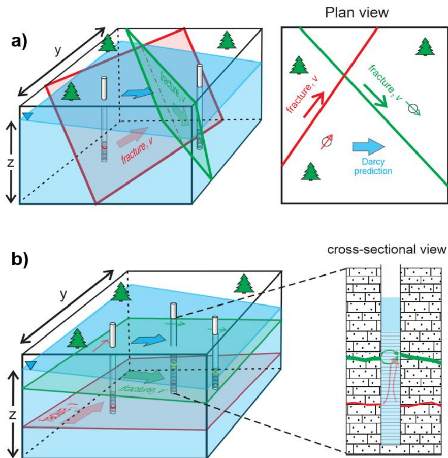
Figure 28 - Simplified schematics of two fracture systems in which the matrix rock is practically impermeable. a) intersecting fractures each with its own flow magnitude and direction, determined by the respective orientations of the fractures, neither of which corresponds to the regional flow determined from Darcy’s Law. b) Non-intersecting fractures in hydraulic isolation except for a cross-cutting borehole. The two fractures have different flow directions and magnitudes, with the upper fracture dominant. Flow enters the borehole from the lower fracture and leaves the borehole through the upper fracture making the measurement of horizontal velocity in the open well problematic.
