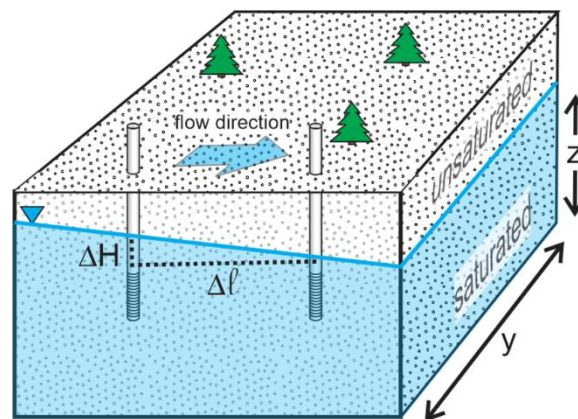
Figure Exercise 2-1 - A lucky hydrogeologist placed two wells in the ground at this site that are aligned perfectly with the flow direction.
