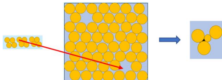
Figure Exercise 1-3 – Drag the small grains into the sample to fill in pores between the larger grains and color in pores that are disconnected from the other pores.
