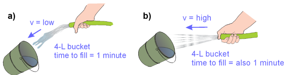
Figure 4 - Water flow from a hose. a) The Darcy flux is the speed (meters per minute) of water flowing from an unobstructed hose. b) The seepage velocity is the speed of water flowing from a hose with an obstructed cross-sectional area. The discharge (liters per minute) is the same in both examples.
