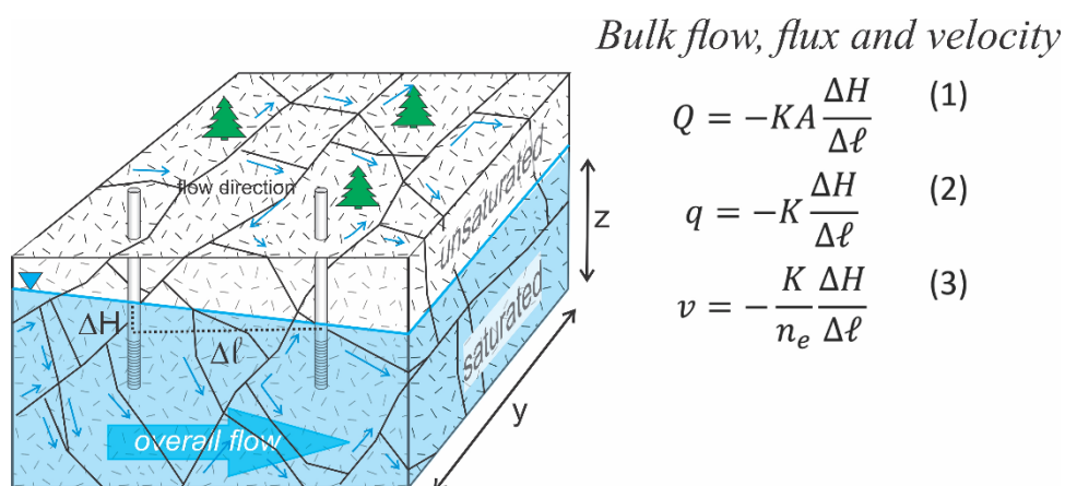
Figure 27 - Conceptual diagram of a fractured rock aquifer showing the difference between flow constrained by the fractures (small blue arrows) and the estimated bulk flow from conventional Darcy's Law calculations (large blue arrow). On a sufficiently large scale, the Darcy calculations will match the average overall flow in the aquifer, including flow direction. On the scale of this diagram severe deviations from the Darcy predictions are evident (small blue arrows) due to locally variable fracture porosity, hydraulic conductivity, and available pathways for flow (also illustrated in Figure 28 ).
