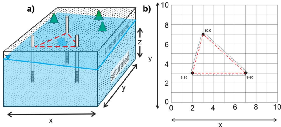
Figure Exercise 2-2 – A conceptualized diagram of an aquifer with a) three wells used to investigate the site in order to estimate both the direction of flow and the velocity; and, b) a map showing the relative positions of the wells and the water level elevation in each well.
