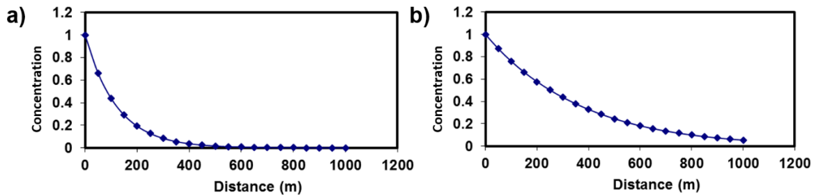
Figure 15 - a) Steady-state plume centerline profile of 1,1 trichloroethane in an aquifer with v = 10 cm/day and t_{1/2} of 2.3 years. Plume size is sufficiently wide and deep that the boundaries do not influence the concentrations on the centerline. b) The same plume steady-state centerline profile with v = 30 cm/day. Prior knowledge of the rate constant (through t_{1/2} ) is not deterministic of the plume size without good knowledge of the groundwater velocity. (In these calculations, longitudinal dispersivity was fixed at 0.1 m, horizontal transverse dispersivity was set to 0.01 m, and vertical dispersivity was set to 0.015 m).
