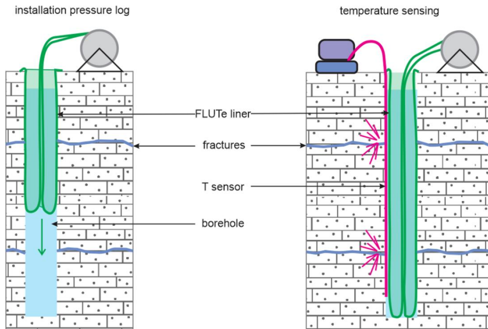
Figure 30 - Schematic of the FLUTE liner as the basis for characterizing fractured media. Both pressure profiles and temperature profiles (using T-sensors) can be used to identify the locations of fractures. The determination of flow rates in the fractures is a further goal for the technology.
