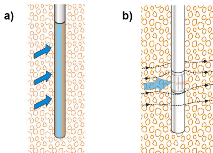
Figure 13 - Schematic diagrams of the a) ISPFS and b) PVP.
