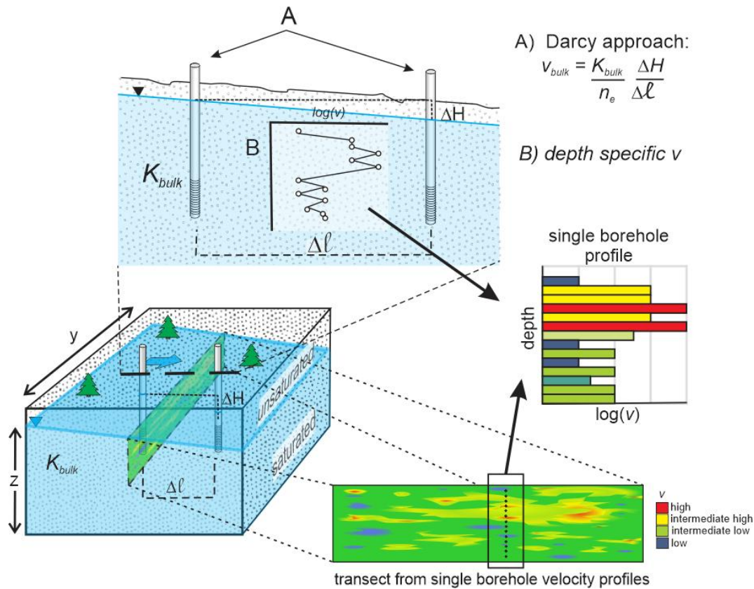
Figure 8 - Comparison of the local velocity information derived from the Darcy calculation and from depth specific velocity measurements. The Darcy approach cannot generally measure small scale hydraulic gradients and therefore produces a velocity value describing the bulk domain. Several single borehole methods are capable of producing vertical profiles of in situ velocity measurements. Previously, this kind of detail was only possible to obtain from grain size analyses or permeameter testing of core materials, and calculations that relied on the ensuing, uncertain estimates of K . Profiles like these can be combined from multiple locations to construct transects, as shown above (only one profile shown, for clarity of illustration). Note: in an actual investigation, the v presented in the transect would be quantitative, rather than the qualitative descriptors in the legend.
