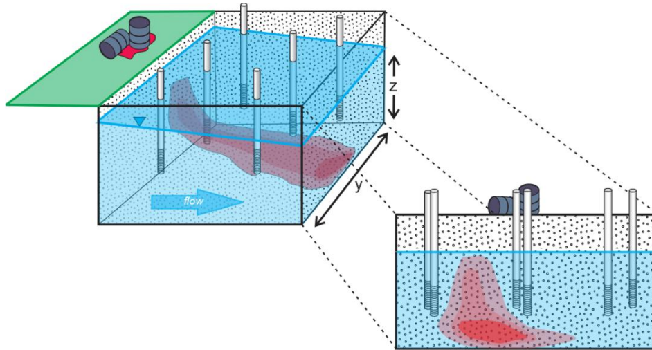
Figure 7 - Illustration showing a multi-well monitor network failing to intersect a plume due to inadequate well spacing and a sinking plume. This scenario could apply to a spill, as illustrated, or tracer tests aimed at characterizing the aquifer — and failing.
