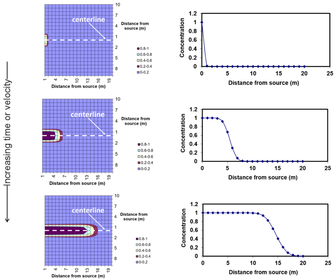
Figure 14 - The growth of a simple plume of groundwater contamination as seen in plan-view with groundwater flow from left to right. The x-axis refers to distance from the source in the direction of flow (longitudinal), and the y-axis refers the distance from the source perpendicular to flow (transverse). In the absence of geological complexities, or pronounced variations in flow over time, plumes will grow into thin, straight zones. Instrumentation along plume centerlines can provide information detailed enough to document plume growth or attenuation in time. In the simulations undertaken to create these images, v was set to 0.04, 0.15 and 0.4 m/d, the longitudinal dispersivity was set to 0.1 m. Horizontal transverse dispersivity was set at 0.01 m and vertical transverse dispersivity was set at 0.0015 m.
