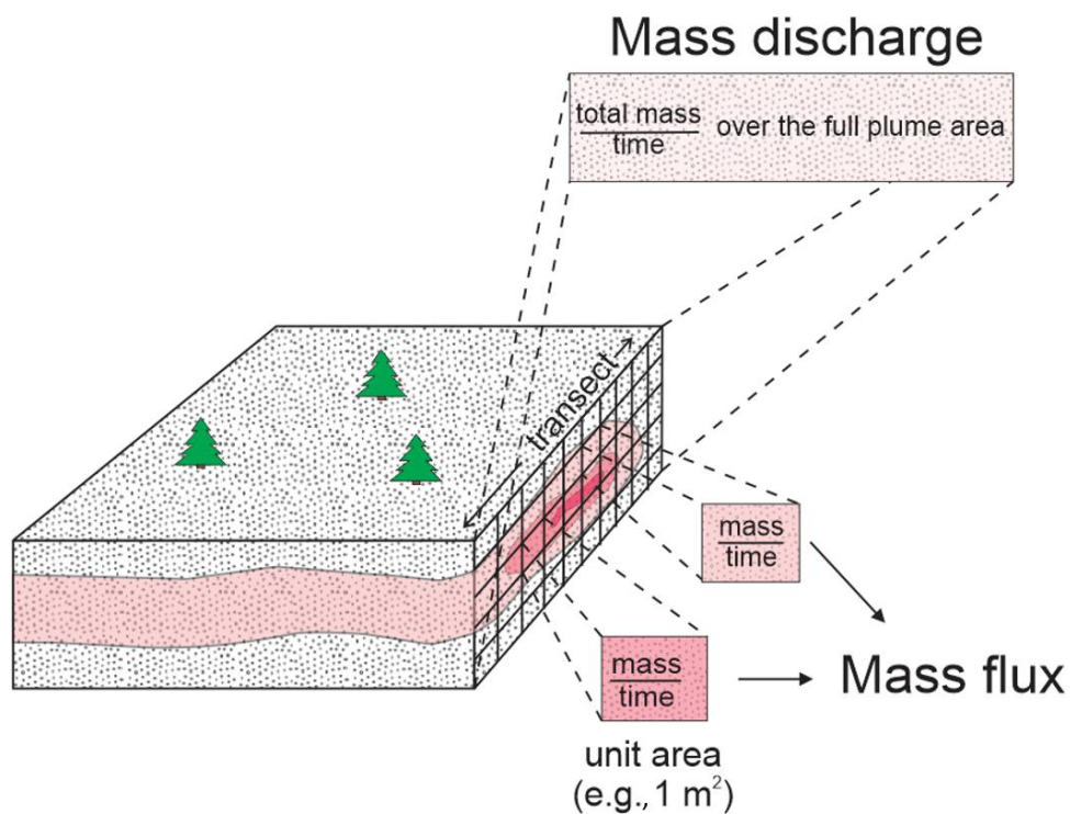
Figure 24 - Relationship between mass flux and mass discharge. Mass flux is the mass of a contaminant that crosses a unit cross-sectional area of an aquifer per unit of time, and it may vary within a plume, as it does between the two example areas shown by the differing colors (dark red and light red). Mass discharge is simply the sum of fluxes over the entire plume.
