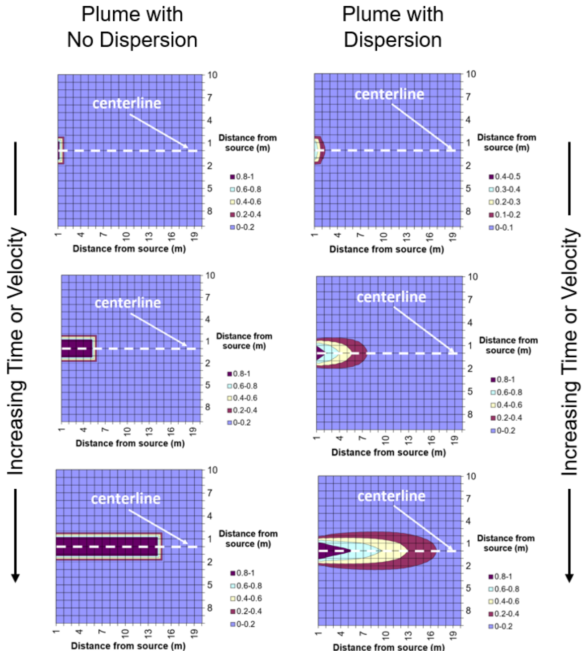
Figure 18 - Plan view of the growth of a simple plume of groundwater contamination with and without the process of dispersion. The plume growing without dispersion illustrates ‘plug flow’ and is purely advective transport. The plume growing with dispersion illustrates the diluting effects dispersion imposes on a plume, as well as extending the volume of aquifer that is contaminated. In the longitudinal direction (the direction of flow), this extension results in slightly earlier arrival times of the pollutant at receptors. These simulations were performed with the same transport parameters as those given in Figure 14 except that the ‘no dispersion’ calculations used dispersivities < 0.001 m, and the ‘dispersion’ calculations used a longitudinal dispersivity of 1 m, a horizontal transverse dispersivity of 0.1 m and a vertical transverse dispersivity of 0.015 m.
