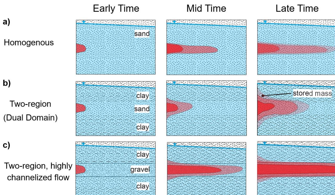
Figure 23 - Conceptualization of plumes being transported in a) a homogeneous sandy medium, b) a heterogeneous medium consisting of sand and clay, and c) a second heterogeneous medium consisting of gravel and clay. Compared to the homogeneous medium, the other two constitute transport in two regions: predominantly advective transport in the sand and gravel layers and mainly diffusive transport in the clay. The effect of the diffusive transport is to store mass and retard the plume compared to the homogenous case. If the clay is coupled with highly permeable sediment (perhaps not known to be present), such as gravel, the advective transport can proceed much faster, overwhelming any retardation that might be expected for the sand-clay coupling.
