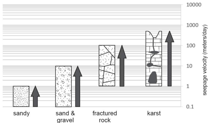
Figure 29 - Approximate, typical seepage velocity ranges for various aquifer settings (John Cherry, Tom Aley, personal communication, 2020). Site specific conditions can extend these ranges for individual cases.
