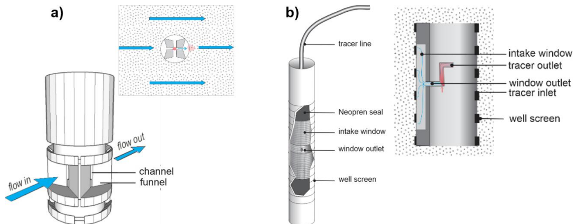
Figure 12 - a) The In-Well Point Velocity Probe. This device is placed in the screened portion of a well where water entering the well is directed through one or two upstream channels. Water leaves the probe through the downstream channels where a tracer, introduced in the center of the probe, is detected. Inset shows a horizontal cross-section to illustrate tracer path from the center of the probe (the release point) through an exit channel, to the aquifer. b) The Direct Velocity Tool. Water is collected in the window and exits through the outlet tube. Tracer is added to the water stream in the tube and is diluted by the stream. The diluted tracer is detected as water leaves the tube. Inset shows a vertical cross-section that illustrates the path of the water entering the collecting window and its direction through the tracer introduction tube.
