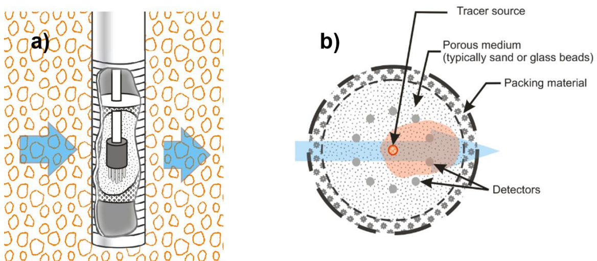
Figure 11 - Schematics of the heat pulse flowmeter. a) Depiction of the instrument packed inside a porous medium within the well. The housing containing the probe is jacketed with a porous material that seals the annular space between the inside of the screen and the probe housing. b) Plan view of the spatial relationships between the tracer release point (center) and the surrounding detectors. Flow is indicated by blue arrows. The tracer pulse is indicated in shades of red.
