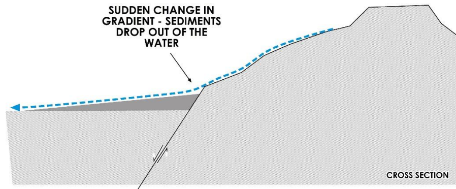
Figure 135 - Cross section of an alluvial fan (dark gray) developing at the foot of a fault-block mountain range where an abrupt change in the stream (dashed blue line) gradient causes rapid deposition of coarse sediment.
