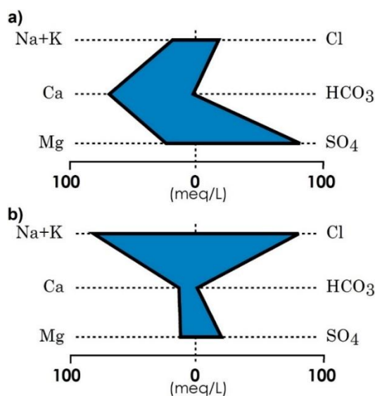
Figure 84 - Stiff diagrams.
