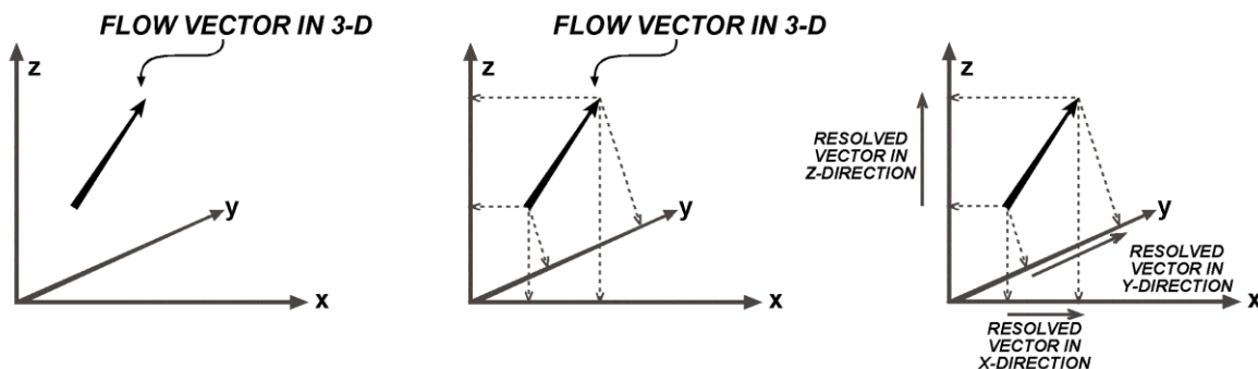
Figure 20 - Vector resolved into component vectors in three dimensions.
