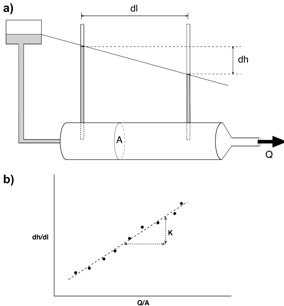
Figure 14 - a) Darcy tube; b) graph showing experimental results.
