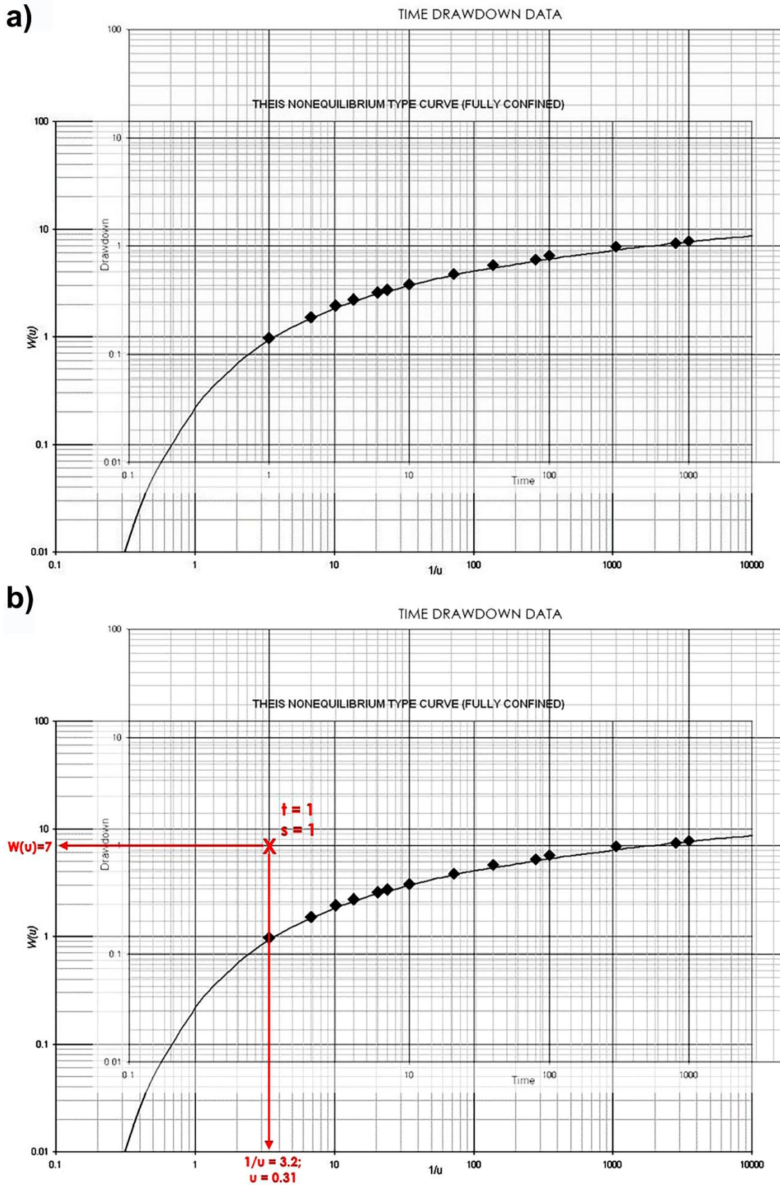
Figure 46 - Example of curve-matching method: a) plotted data overlain on type curve with best match of the data to the type curve; b) match point t (time) = 1 and s (drawdown) = 1 on data graph corresponds to W(u) = 7 and u = 0.31 .
