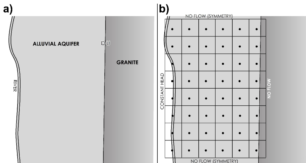
Figure 73 – a) Map of an alluvial aquifer, bounded by a river to the west and a fault-block granite to the east; and b) discretization of the alluvial aquifer with boundary conditions and model nodes.
