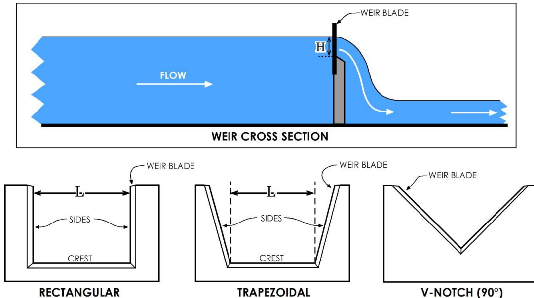
Figure 107 - Different types of weirs.
