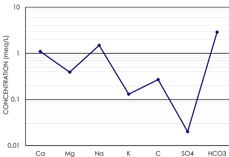
Figure 89 - Schoeller diagram.
