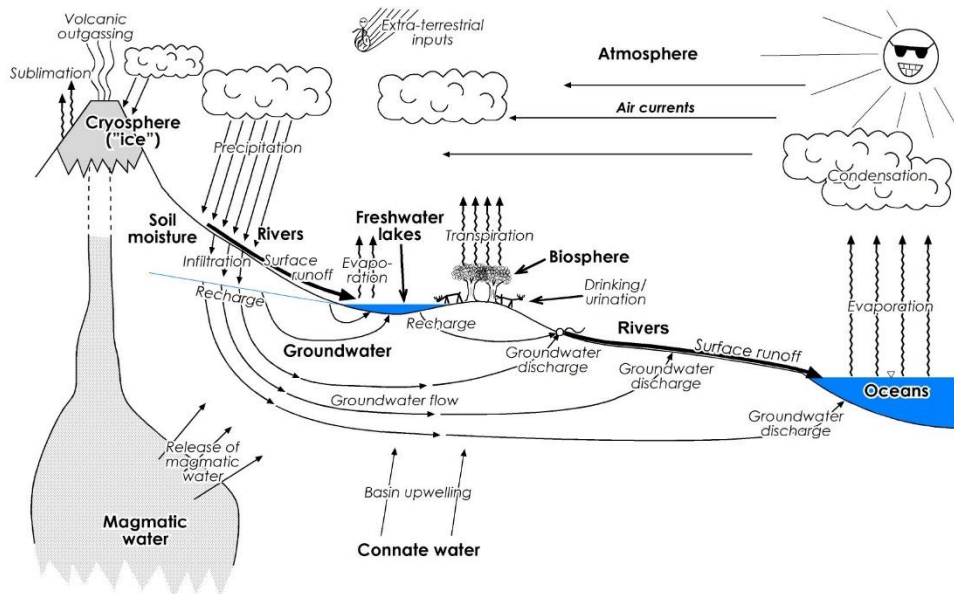
Figure 3 - A generalized and simplified diagram of the hydrologic cycle. Arrows show movement of water within and between reservoirs with straight lines representing movement of liquid and wavy lines represent movement of vapor .
