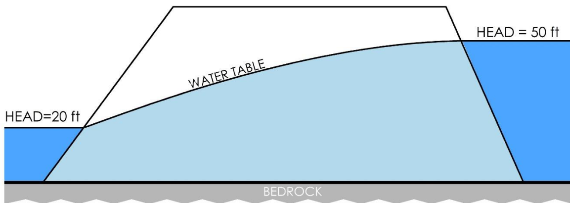
Figure 33 - Cross section showing flow through an earthen dam.
