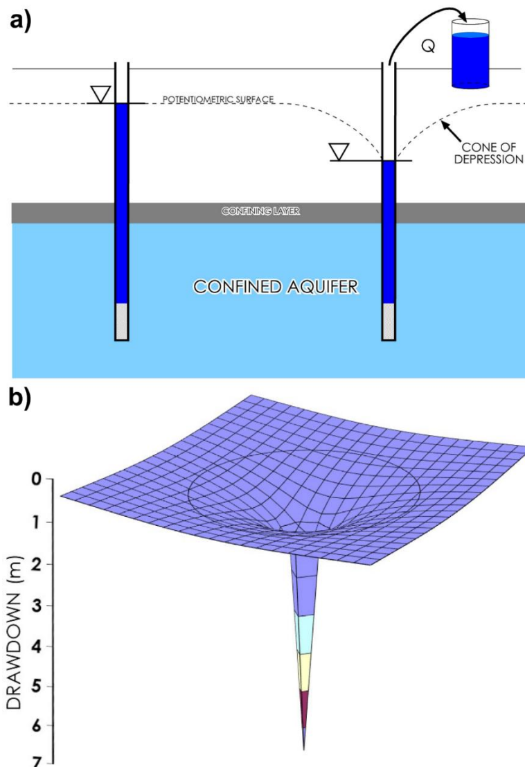
Figure 24 - a) Changes in the potentiometric surface in response to pumping from a well in a confined aquifer; b) 3-D view of a typical cone of depression centered around a pumping well.
