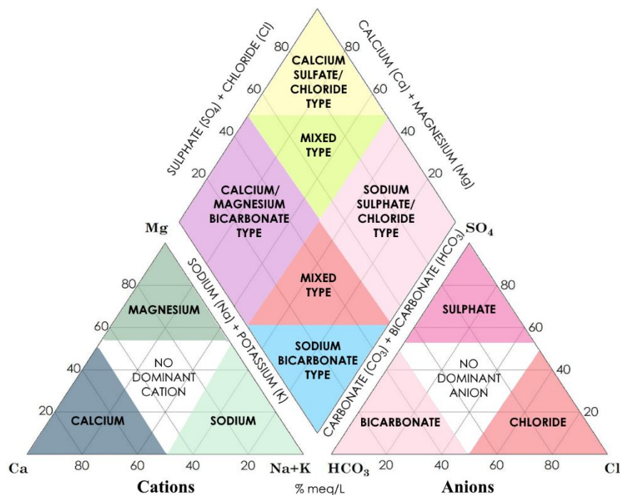
Figure 82 - Water types as delineated by the location of a water analysis on a Piper diagram (modified from Hatari Labs).
