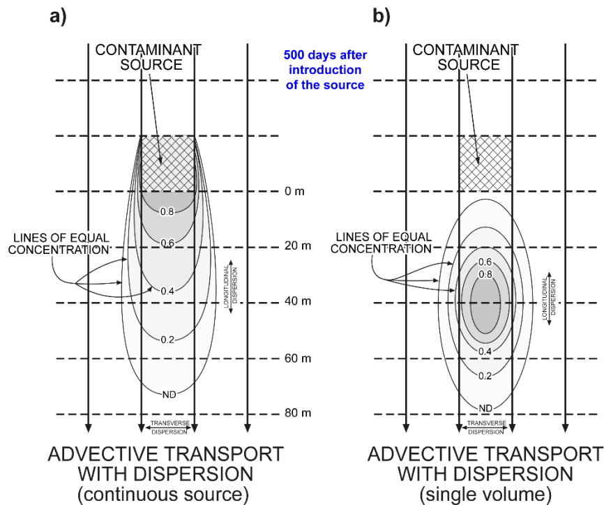
Figure 93 - Advective transport at groundwater velocity of 0.1 m/d with dispersion, showing concentrations relative to initial concentration in the groundwater 500 days after the release of contaminants for the case of a) a continuous source and b) a single volume pulse.
