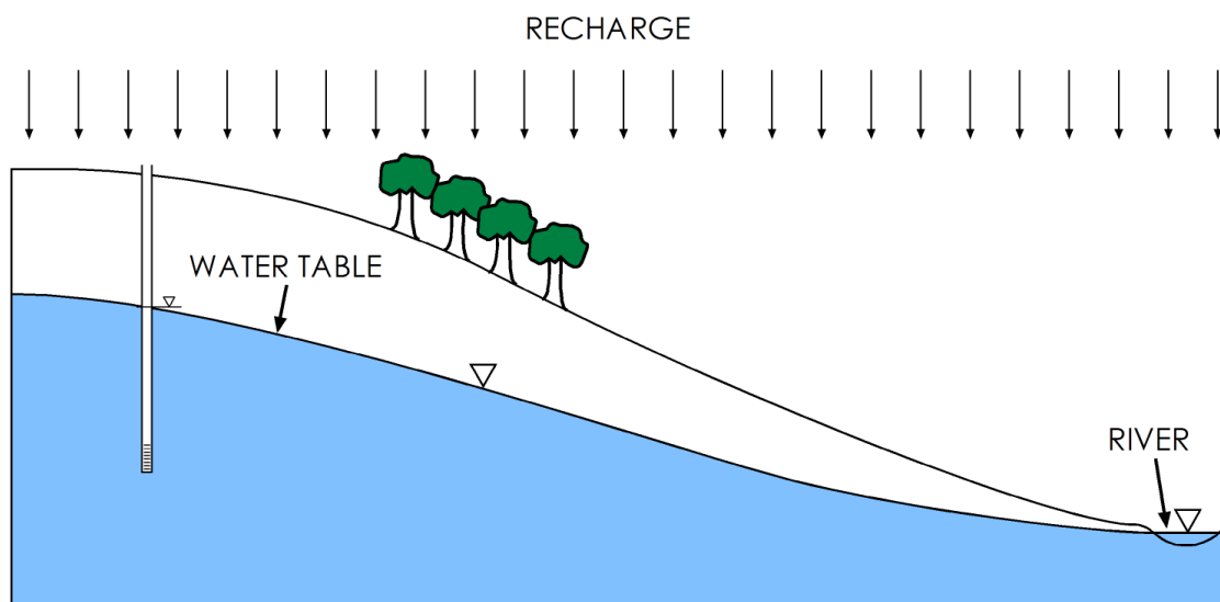
Figure 21 - Unconfined aquifer.
