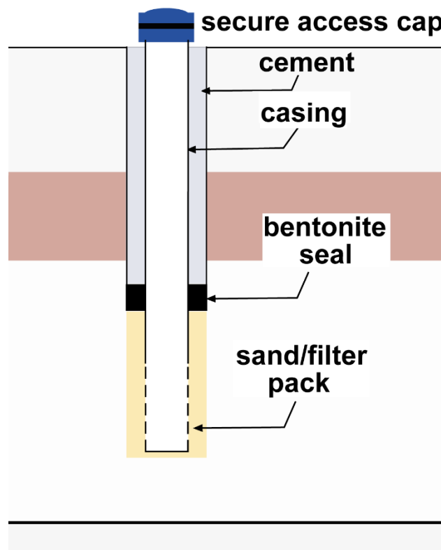
Figure 35 - Typical monitoring well construction.
