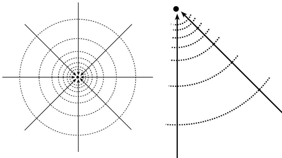
Figure 36 - Radial flow to a well. The dashed lines are equipotential lines that are lowest closest to the well, which is represented by the dot in the center.
