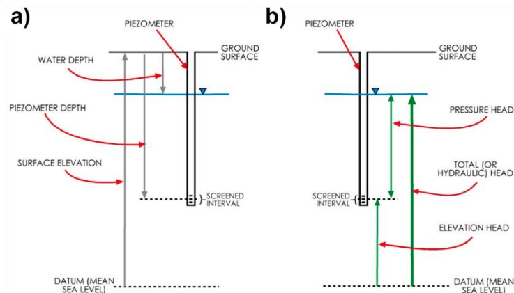
Figure 8 - Hypothetical well showing depths, elevations, and heads.
