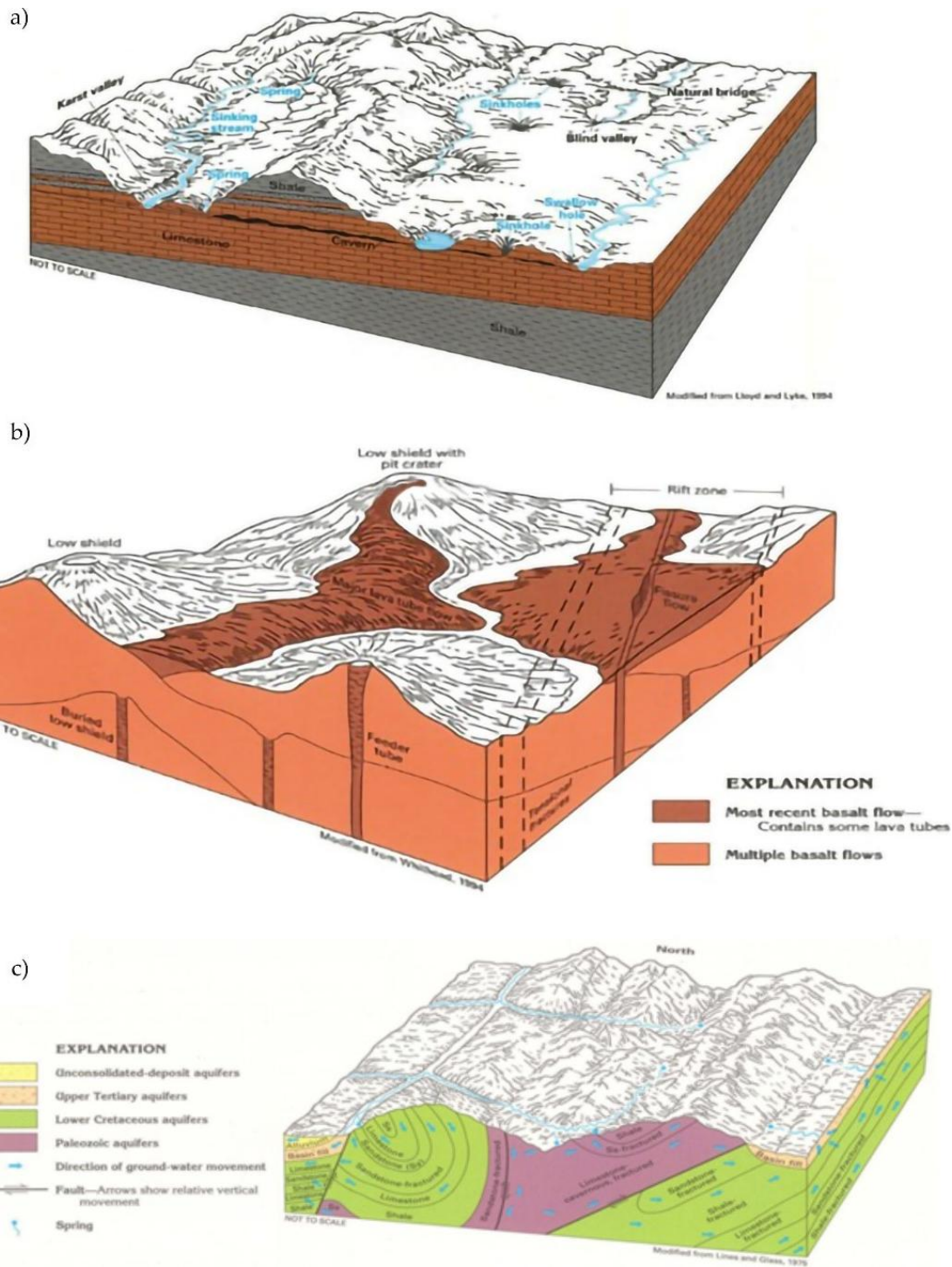
Figure 4 - Three lithologically different consolidated aquifer systems in typical geological settings. a) Karstic limestone aquifer with associated land-surface features such as springs, sinkholes, karst valleys and sinking streams (after USGS, 2000). b) A thick complex of overlapping flows of basaltic lava extruded from numerous overlapping shield volcanoes (Southern Idaho). Most flows issued from a central vent or fissure and some are associated with large rift zones in the Earth’s crust (after USGS, 2000). c) Structurally affected groundwater system consisting of sandstones, shale and limestones (after Whitehead, 1996).
