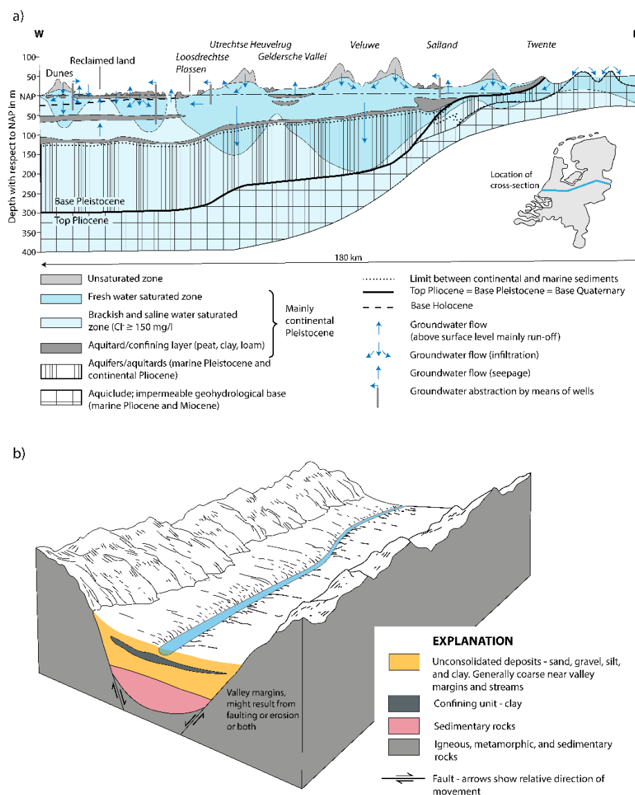
Figure 3 - Two examples of sand and gravel aquifers in different geological settings: a) a hydrogeological cross-section through The Netherlands showing a multi-layer aquifer system in a subsiding geological basin, bordered at its western margin by the North Sea (Dufour, 2000); and, b) a conceptualization of a basin-fill aquifer (USGS, 2000).
