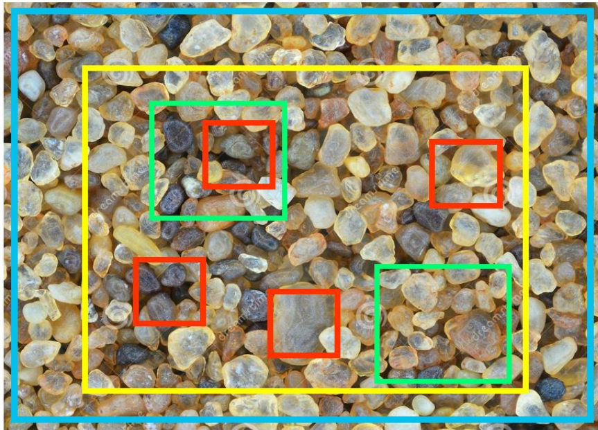
Figure 1 - Demonstration of the concept of 'Representative Elementary Volume (REV)' of a porous medium (here shown in 2D projection). Explanation: With increasing size, the observed porosity (or void ratio) of a control volume changes from meaningless for macroscopic analysis (red boxes or smaller) to meaningful and representative (large blue box). Intermediate sizes may yield poorly (green boxes) to nearly representative porosity values (yellow box) for the medium considered.
