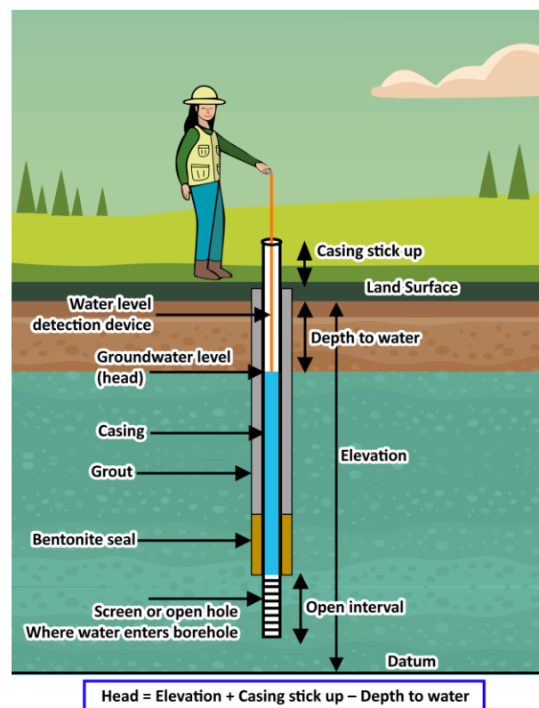
Figure 2 - Water-level monitoring well showing well features and equation for calculating head. There may be a sand pack (not shown) around the screen, but not around an open hole.
