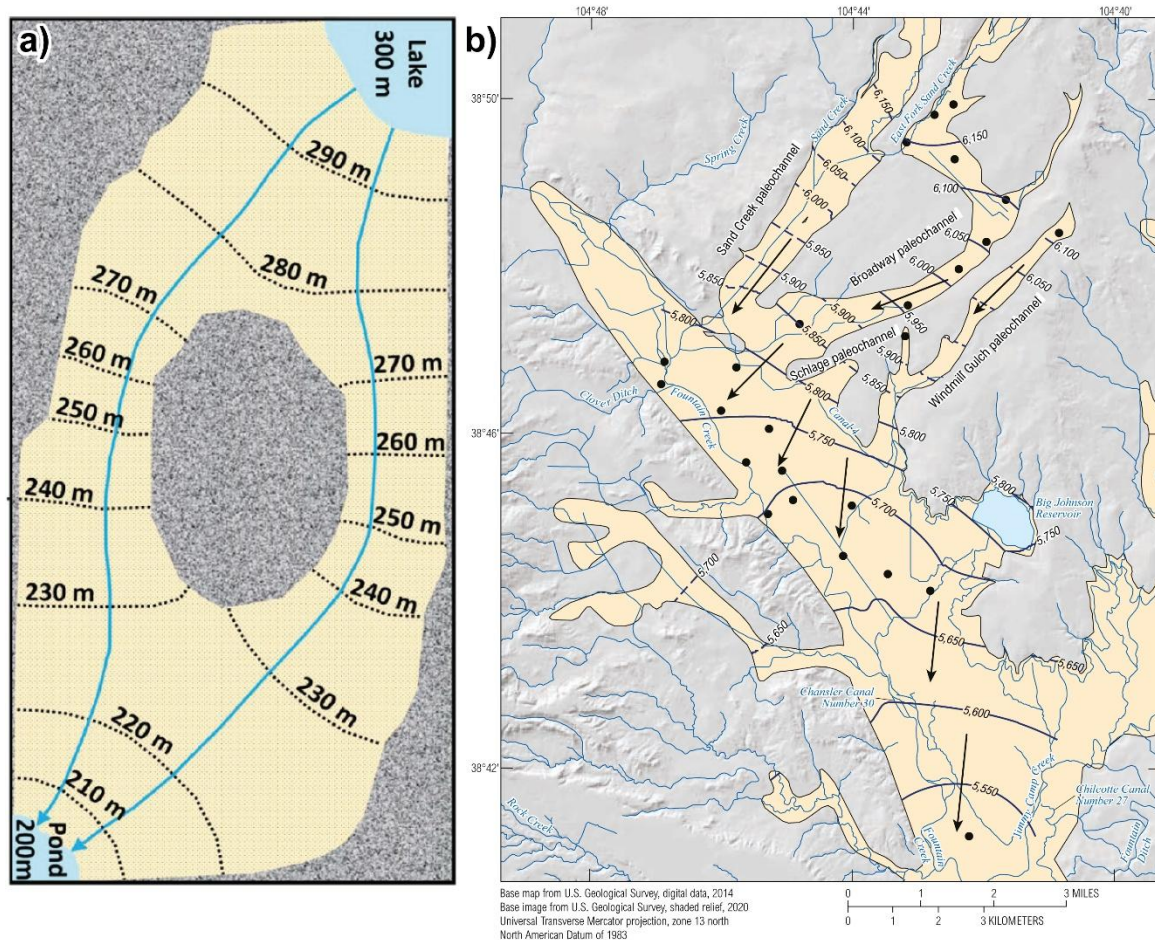
Figure 16 - Influence of a bedrock boundary along an alluvial aquifer. a) A constructed groundwater flow net (from Poeter & Hsieh, 2020). b) A contour map of measured groundwater head (from Newman and others, 2024), in feet with 6150 ft \approx 1875 m and 5550 ft \approx 1692 m. In this example the authors inferred no leakage between the bedrock and the alluvium along the elongated lobes in the north where contours are drawn perpendicular to the boundary, but inferred leakage across the bedrock boundary in the broad alluvial valley as indicated by the curved contours that are not perpendicular to the bedrock-aquifer boundary.
