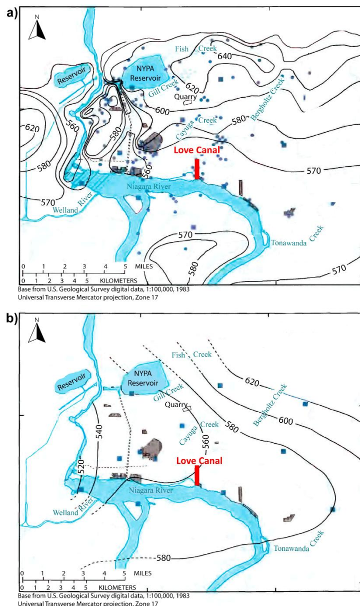
Figure 4 - Head maps of a) the shallow (overburden) and b) deep (dolomite) aquifer in the Niagara Falls area (modified from Yager, 1996). The Love Canal landfill is located along the river. Contours of head are in feet (600 ft \approx 183 m, and 20 ft \approx 6 m); and wells are noted as either circles or squares. The contour values are generally lower in the deep aquifer. The direction of flow differs in the two aquifers as determined by envisioning flow to be approximately perpendicular to the contour lines.
