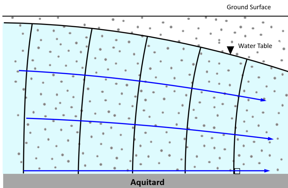
Figure 24 - Mainly horizontal flow in an unconfined aquifer. The potentiometric contours are orthogonal to the aquitard, which has a very low hydraulic conductivity ( K ) such that it behaves as a no-flow boundary (Cohen and Cherry, 2020).
