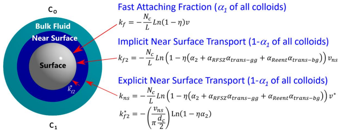
Figure 47 - Upscaling algorithm for unfavorable conditions (from Johnson, 2020).
