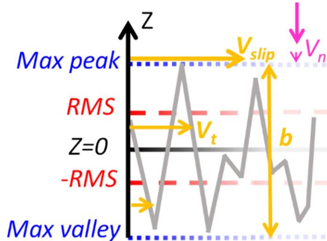
Figure 26 - Schematic of parameters modified in the impinging jet model to account for slip, with the explicit rough surface represented by the jagged gray line. The continuum expressions for v_t are a function of z + b , with b = 0 for smooth surfaces. For rough surfaces, the no-slip condition for the normal component v_n occurs at the effective contact plane and the no-slip condition for the tangential component v_t occurs at distance b below the effective contact plane. The slip velocity ( v_{slip} ) is the finite tangential fluid velocity at the effective contact plane (a plane lying on the highest asperity tops, i.e., labeled Max peak in the image).
