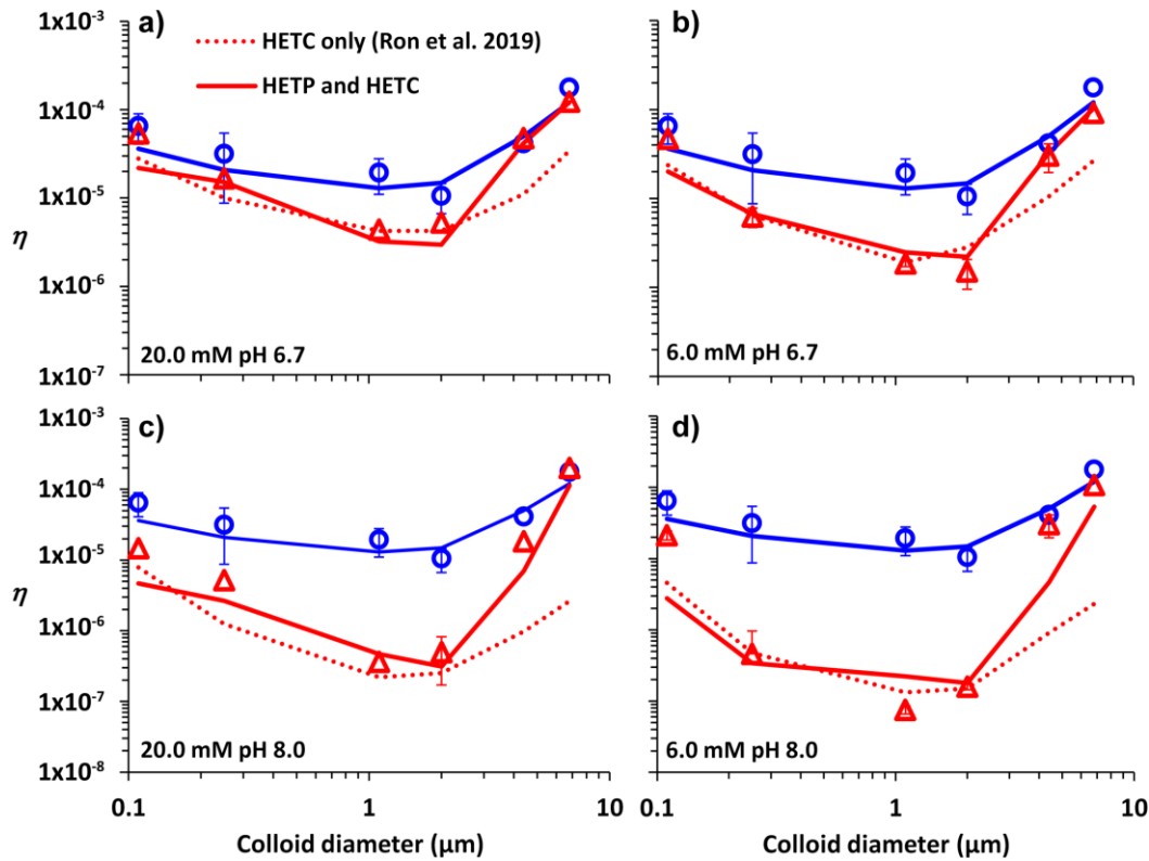
Figure 17 - Experimental (symbols) versus simulated (lines) trends of collector efficiency as a function of colloid diameter under favorable (blue) versus unfavorable conditions (red). Efficiency varies depending on ionic strength and pH: a) IS 20 mM and pH 6.7, b) IS 6 mM and pH 6.7, c) IS 20 mM and pH 8, and d) IS 6 mM and pH 8. The surface is silica and the colloids are carboxylate-modified polystyrene latex microspheres. For colloids between the 1 to 2 \mu\text{m} diameter size, the gap between favorable and unfavorable collector efficiencies ( \eta ) is greatest. This gap decreases for smaller and larger colloid sizes outside the n - \mu transition. Repulsion (and the gap between favorable and unfavorable ( \eta )) increases with increased pH and the associated decreased IS in this system. Simulations were performed for nanoscale heterogeneity on the collector only (HETC) and for nanoscale heterogeneity on both the collector and the colloid (HETP) (from Pazmiño et al., 2014; Ron et al., 2020).
