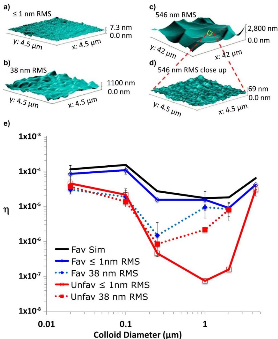
Figure 18 - Atomic force microscopy (AFM) nano topography of samples with increasing root mean squared (RMS) roughness: a) < 1 nm, b) 38 nm, and c) 546 nm, with d) showing a close-up of (c). e) Collector efficiency as a function of colloid size for different values of RMS roughness under favorable and unfavorable conditions, as well as simulated under favorable conditions (Fav Sim; from Rasmuson et al., 2017).
