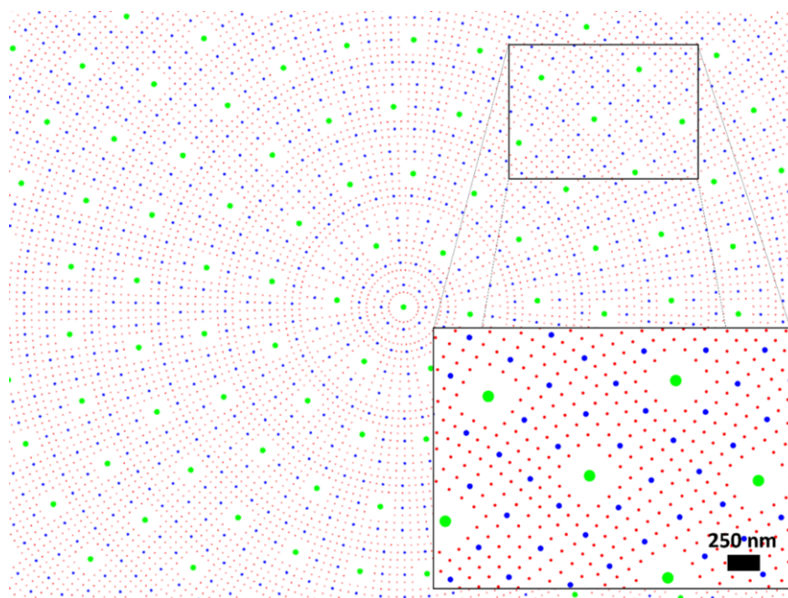
Figure 32 - Representation of DRNH (discrete representative nanoscale heterogeneity) on the collector surface. HETC (heterogeneity on the collector surface only) were represented by three R_{HETC} : 90 (green), 45 (blue), and 25 (red) nm with spatial frequency ratios of 1, 8, and 64, respectively. All three HETC were present on the simulated collector surface. In this representation, SCOVC (surface coverage colloid) was increased for visualization purposes.
