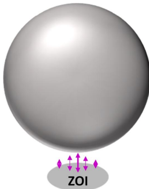
Figure 9 - Zone of colloid-surface interaction (ZOI) between a colloid (denoted by sphere) and an implied flat surface on which the ZOI (shaded circular area) is shown. xDLVO interactions are integrated across this zone. Only normal interactions are considered. The magnitudes of the interactions are denoted by the lengths of the magenta double-headed arrows, which are largest at the location of smallest separation distance between the surfaces.
