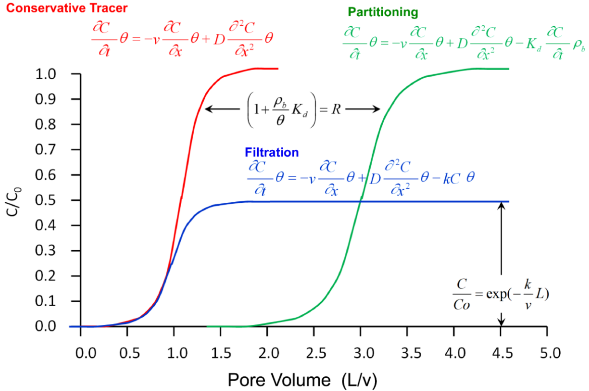
Figure 42 - BTCs for a conservative tracer (red), partitioning solute (green), and irreversibly lost solute or colloid (e.g., filtration; blue) (after Hunt & Johnson, 2016).
