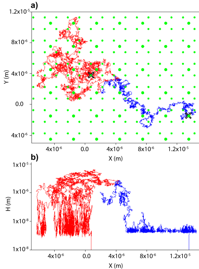
Figure 37 - a) Plan view and b) cross view of two representative colloid trajectories under unfavorable conditions over a collector surface (located at H=0 in b). The 0.25 μm colloid (red) is more mobile due to increased diffusion and its behavior resembles a mosquito. In contrast, the 1.95 μm colloid (blue) has reduced diffusion and a deeper secondary energy minimum, which results in less vertical mobility and slow lateral movement while near the surface, resembling the tracking behavior of a bloodhound.
