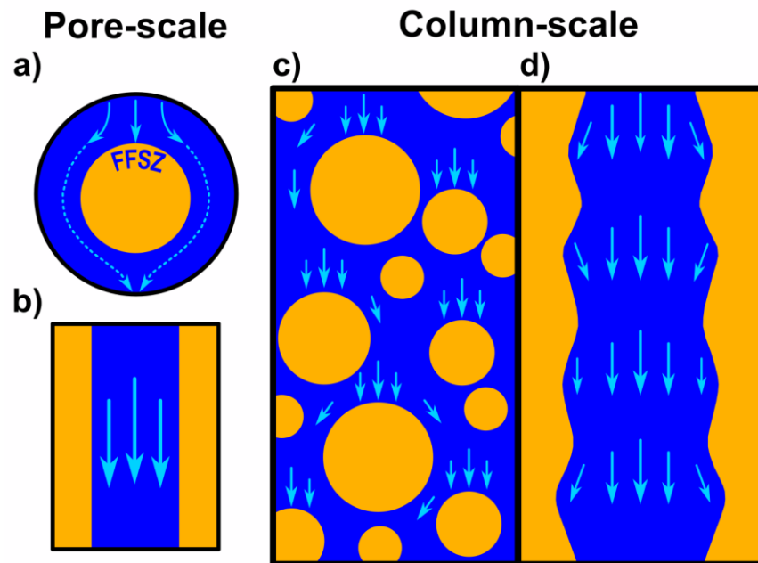
Figure 54 - Contrasting colloid transport simulation geometries at the pore scale in a) granular versus b) fractured media and at the column scale in c) granular versus d) fractured media (modified from Rasmuson et al., 2019b).
