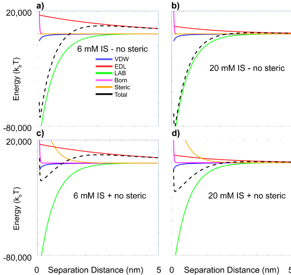
Figure 8 - Influence of xDLVO interactions in the primary energy minima: a) and b) show negligible influence of IS increase in the primary minima depth, c) and d) show the effect of steric interactions. Energy minima depth is reduced by a factor of approximately 4 due to the increased repulsion. The IS influence is more noticeable. In all cases Lewis AB interactions are the most important contributions to the minima depth. For this reason, there is not a clear shift of the primary minimum location in response to steric repulsion.
