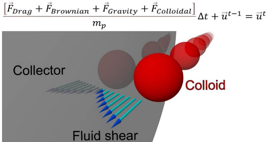
Figure 19 - Representation of colloid trajectory simulation obtained from a force balance. At relatively longer separation distances ( > 200 nm) where colloidal forces are negligible. Once the colloid is near the surface ( < 200 nm), colloidal forces play a critical role in colloid attachment (immobilization in contact), retention (weak association in the secondary energy minimum in zones of small fluid shear), and re-entrainment back to the bulk fluid.
