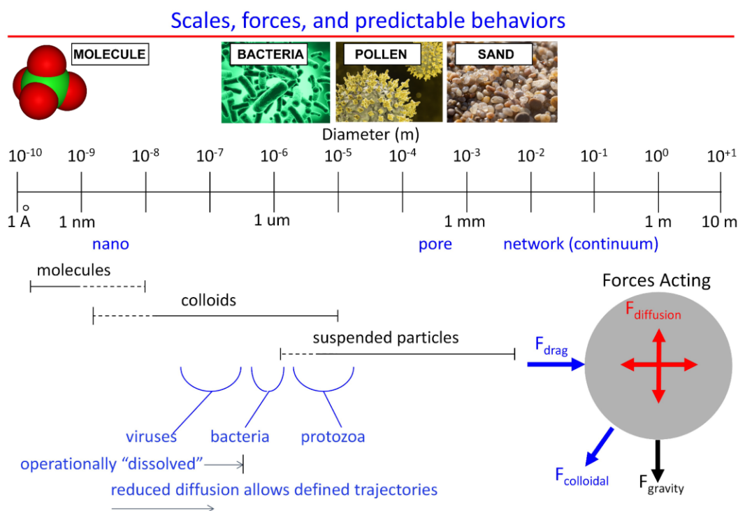
Figure 4 - Colloidal particle size range encompasses many orders of magnitude. Particle size has a great influence on the forces acting on the particle. Smaller colloids tend to behave as molecules (with increased diffusion) while larger ones tend to settle. Both processes are less influential on intermediate-size colloids, which are generally the most mobile.
