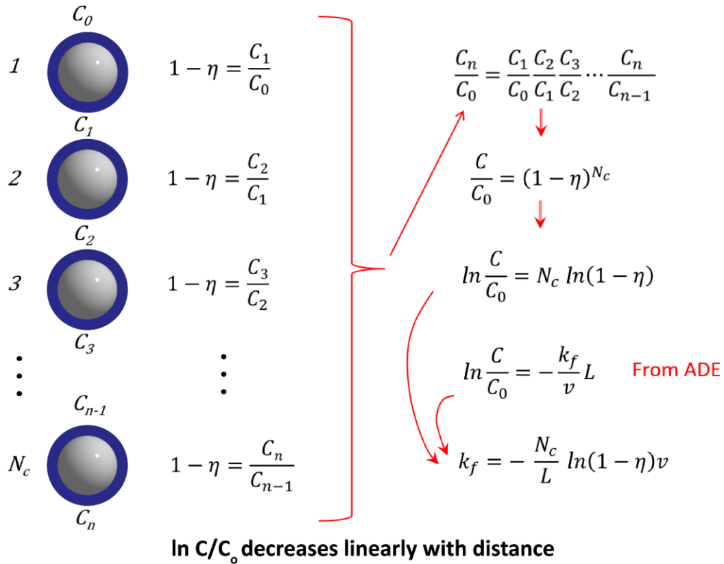
Figure 43 - Upscaling from pore-scale collector efficiencies ( \eta ) to continuum-scale rate coefficients ( k_f ) where ADE is the advection-dispersion equation.
