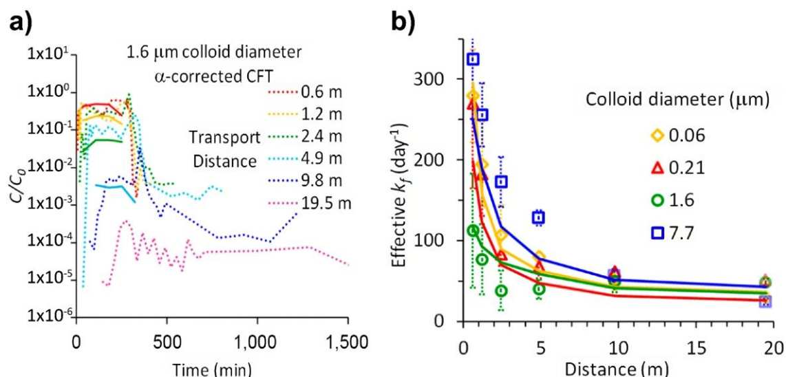
Figure 40 - Breakthrough-elution concentration histories in pea gravel for carboxylate-modified polystyrene latex colloids (1.6 \mu\text{m} diameter) with experimental results shown by dotted lines colored according to transport distance. a) Steady-state breakthrough according to \alpha -corrected colloid filtration theory is shown by solid-colored lines, with \alpha determined from the 0.6 m transport distance. b) Values of effective k_f as a function of transport distance determined from experimentally observed steady-state breakthrough (shown by symbols) with error bars representing error propagation as described in Johnson and others (2020). Solid colored lines in (b) show values of k_f from upscaling of mechanistic pore-scale trajectory simulations incorporating representative nanoscale heterogeneity, which is described in Section 6.2 (modified from Johnson et al., 2020a).
