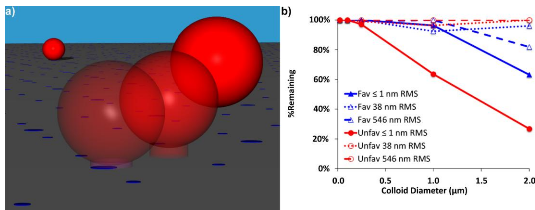
Figure 46 - Colloid re-entrainment after high flow perturbation. a) Schematic of colloid (red spheres with ZOI shown as a cylinder initially over a blue heterodomain) re-entrainment in response to increased fluid drag under unfavorable conditions. b) Percent remaining on various surfaces after high flow perturbation ( 0.15 \text{ ms}^{-1} ) for colloids loaded under the 1.7 \times 10^{-3} \text{ ms}^{-1} velocity condition (from Rasmuson et al., 2017).
