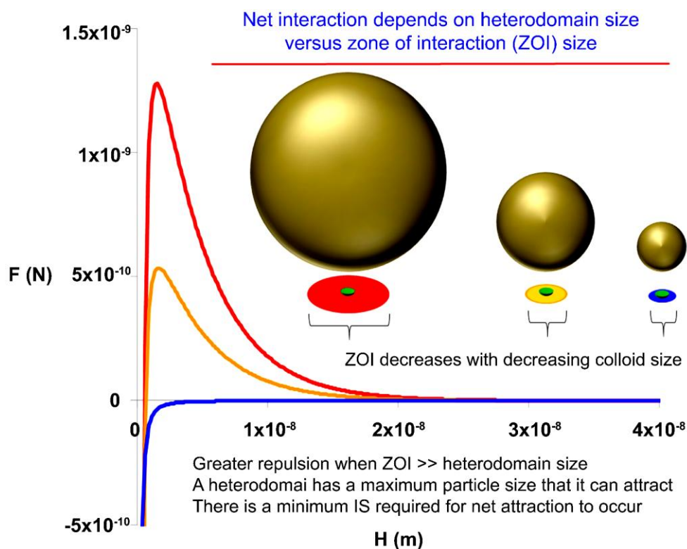
Figure 10 - Colloid-heterodomain interactions as a function of colloid size. Colloids are depicted as gold spheres interacting with an implied surface below the sphere across a zone of interaction (ZOI) depicted by red, yellow, and blue disks that, for a given solution ionic strength (IS), are proportional in size to the colloid. An area of charge heterogeneity on the surface is depicted as green disks. The greater the fraction of ZOI occupied by heterodomain, the lesser the repulsive barrier as depicted force profiles ( F ) versus colloid-surface separation distance ( H ) using colors (red, yellow, and blue) for the ZOI of the three colloid sizes. Positive values of F are repulsive, while negative values are attractive.
