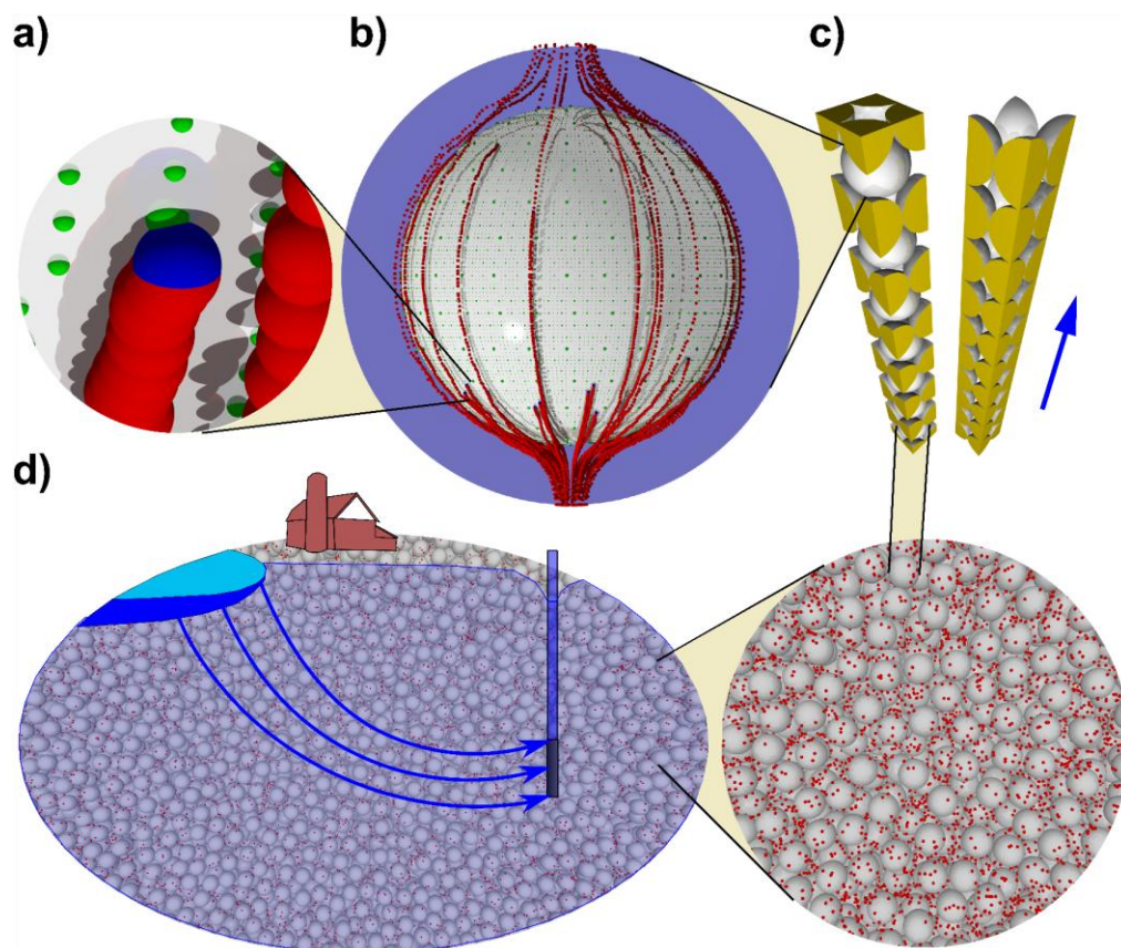
Figure 2 - Schematic of the range of scales involved in colloid transport in groundwater. Scales range from a) nanoscale where colloids (transitioning from red for mobile to blue for attached) interact with charged heterogeneities (green) on grain surfaces (white), as simulated at b) the pore scale in representative collectors (grain plus fluid shell) that in series represent c) a granular media. The transport characteristics determined via simulation in representative collectors are upscaled to continuum-scale rate coefficients to represent d) transport in granular media at the laboratory column and field scales.
