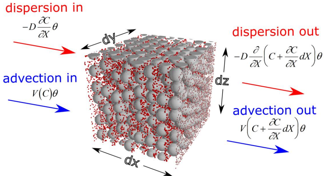
Figure 41 - Control volume to perform mass balance in derivation of the advection-dispersion equation. Gray spheres represent grains; red spheres represent solute.
