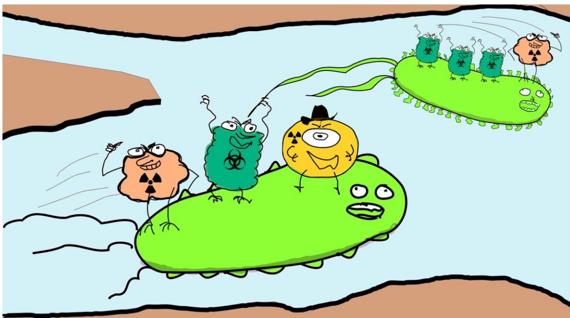
Figure 3 - Schematic of facilitated transport of hazardous solutes via solute-colloid association (heavily inspired by McCarthy & Zachara, 1989).
