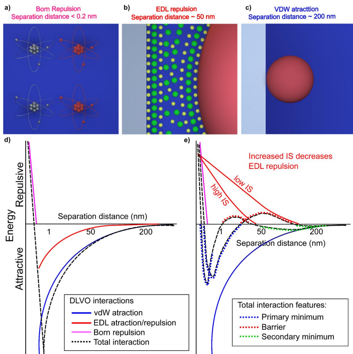
Figure 7 - Colloid-surface (DLVO) interactions. Schematized Born, EDL, and VDW interactions between colloid (red) and grain (gray) surfaces (IS is ionic strength): a) electron orbital overlap, b) counterion-counterion interaction, and c) instantaneous bond dipole interaction. Schematics are scaled according to maximum reach of the interaction. Graphs show DLVO interaction profiles arising from superposition of Born, EDL, and VDW, interactions: d) DLVO profile with attractive EDL interactions (from oppositely charged surfaces) show an attractive primary minimum and absence of a repulsive barrier, e) DLVO profiles show repulsive EDL interactions (from like-charged surfaces) with a relatively shallow primary minimum and a repulsive barrier. The depth of the primary minimum increases, and the height of the repulsive barrier decreases, with increased ionic strength.
