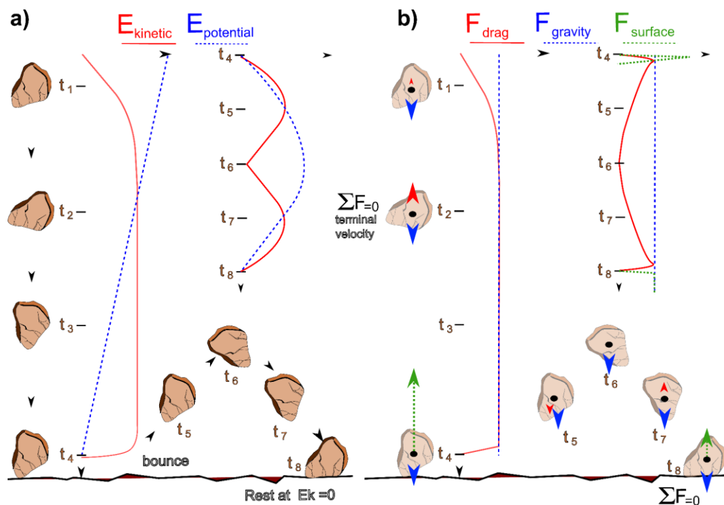
Figure 5 - a) Potential and kinetic energy of a falling particle. b) Forces acting on falling particle. At time t_1 , the particle starts to fall in response to gravity with potential energy below its starting value and relatively small kinetic energy corresponding to relatively low velocity. Friction with air yields a drag force that opposes motion. As the particle accelerates, potential energy is converted to kinetic energy, and the drag force increases with velocity. Maximum (terminal) velocity is reached once the drag force equals the gravitational force ( t \geq t_2 ) after which its kinetic energy remains constant and the drag force equals the gravitational force. At impact ( t = t_4 ), potential energy is minimum (local reference level) and kinetic energy is transferred to the surface. The surface force (a combination of elastic and action-reaction forces) lifts the particle, converting kinetic to potential energy, and the drag force opposes upward motion ( t - t_5 ). Once lift and drag forces equal zero ( t = t_6 ), the overall process repeats until the particle comes to rest in a stable equilibrium ( t_8 ) with net force zero and overall energy minimized.
