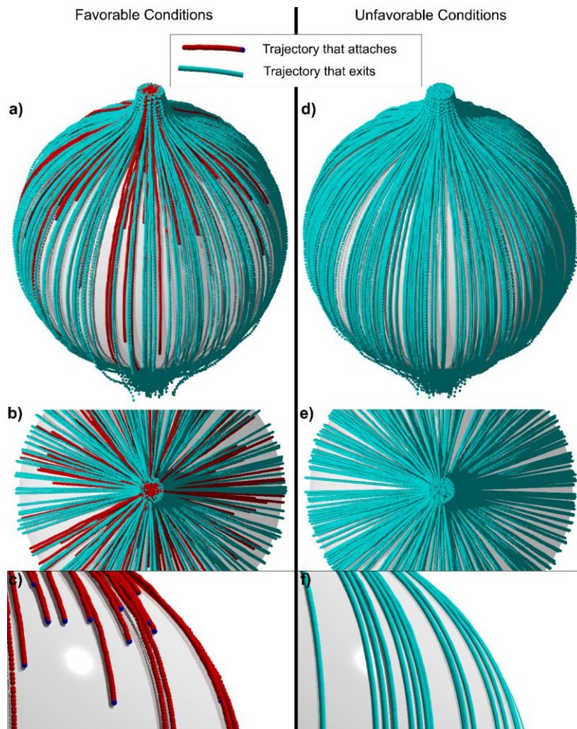
Figure 15 - Simulated colloid trajectories in a Happel sphere-in-cell collector lacking nanoscale charge heterogeneity with flow from top to bottom for favorable conditions (a, b, and c) and unfavorable conditions (d, e, and f). Trajectories are red for colloids that attach and cyan for colloids that exit without attachment. Three views are provided: distant side view (a and d), top downward view (b and e), and close side view of trajectories that attach under favorable conditions (c and f).
