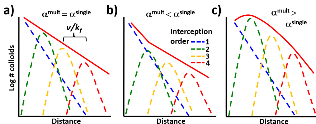
Figure 52 - Schematic RPs (solid red line) for a) exponential, b) multiexponential, and c) nonmonotonic. Dashed lines indicate single and multiple intercepting attached colloid RPs, with color warmth corresponding to increased interception order. The average pore water velocity ( v ) relative to the interception rate coefficient ( k_f ) defines a characteristic spacing between peaks in the RPs for multiple interception attachers (from Johnson et al., 2025).
