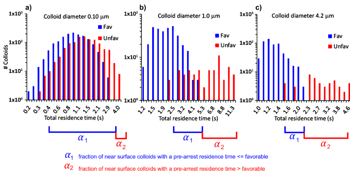
Figure 48 - Histograms of pore scale (Happel sphere-in-cell) simulated total residence times prior to attachment for the three, contrasting carboxylate-modified polystyrene latex colloids of three sizes in fine sand, a) 0.1 \mu\text{m} , b) 1.0 \mu\text{m} , and c) 4.2 \mu\text{m} (from Johnson, 2020).
