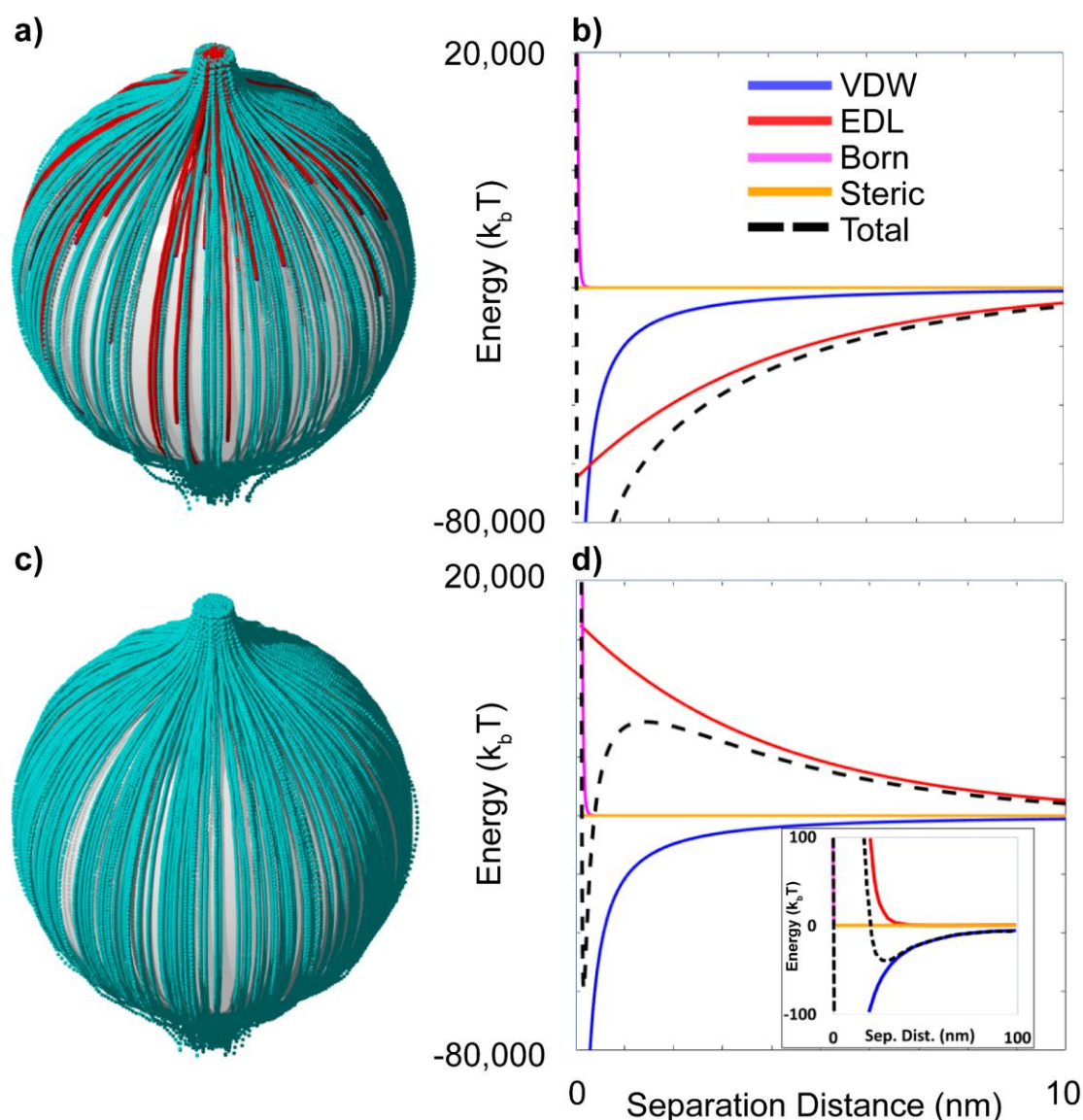
Figure 30 - a) Trajectory simulation with attachment trajectories in red and exit trajectories in cyan in the Happel unit cell and b) DLVO energy profiles for favorable conditions in contrast to c) and d) for unfavorable conditions. Under favorable conditions, there is no repulsive barrier to prevent attachment, and so colloid trajectories that are in near-surface fluid result in attachment. In contrast, under unfavorable conditions lacking nanoscale charge heterogeneity, a significant repulsive barrier ( \approx 8000 k_b T ) prevents attachment, whereas secondary minimum attraction (inset of (d)) associates near-surface colloids with the grain surface such that they translate slowly downgradient in the near-surface domain (without contact).
