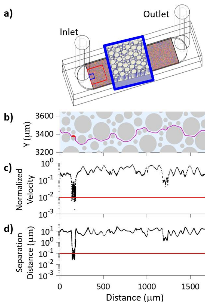
Figure 51 - a) 2D flow cell used for experiments and mechanistic trajectory simulations (Johnson et al., 2025), with b) example colloid trajectory; c) colloid velocity normalized to maximum velocity; and d) separation distance (lower right).
