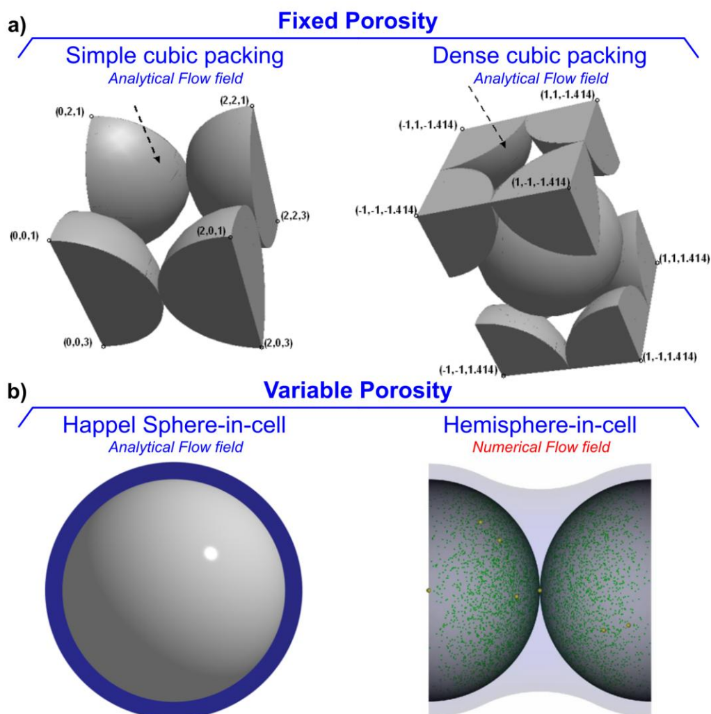
Figure 20 - Most common unit cells used in pore-scale colloid transport simulations: a) variations of fixed packing, and b) variable porosity.
