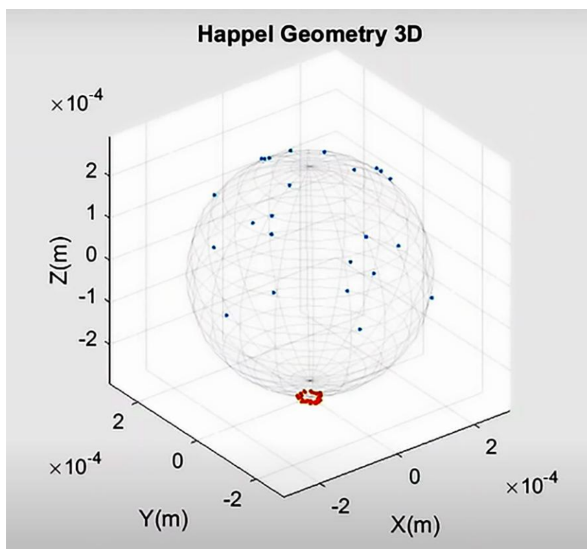
Figure 25 - A video introducing determination of collector efficiencies in Parti-Suite can be watched by clicking the white arrow in the middle of the figure and the subsequent video symbol "▶", or clicking here YouTube .
