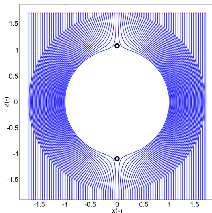
Figure 21 - Two-dimensional representation of Happel sphere-in-cell collector flow field streamlines. A uniform flow field (downward) exists outside the Happel fluid shell (shown for porosity = 0.85 for clarity). Streamlines diverge around the upstream hemisphere and converge around the downstream hemisphere, forming forward and rear flow stagnation zones indicated by small black circles in the upstream and downstream hemispheres, respectively.
