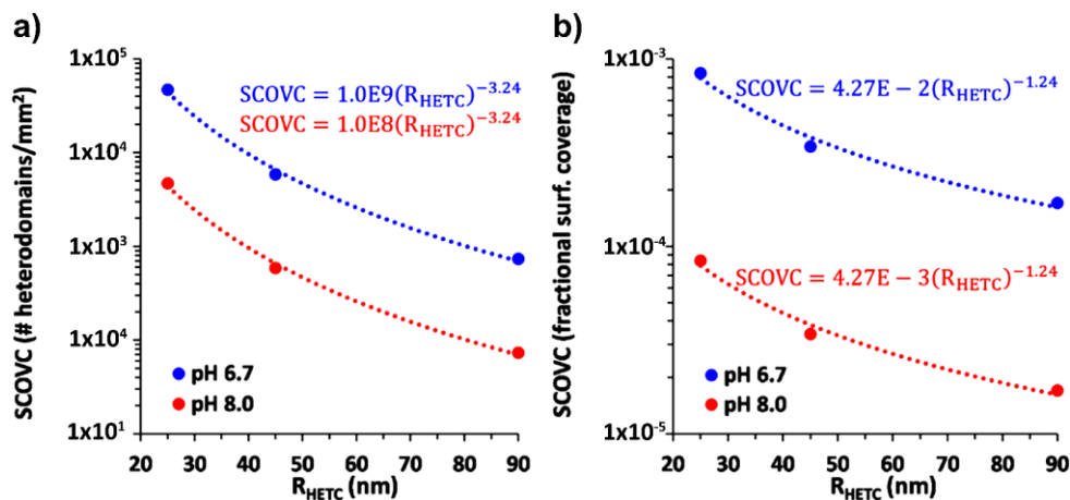
Figure 31 - Discrete representative nanoscale heterogeneity (DRNH) distributions utilized in colloid trajectory simulations with surface coverage (SCOVC) as a function of radius of heterodomains on a) the collector ( R_{HETC} ) expressed as number per area and b) fraction of total surface area. Heterodomain size distribution follows a power law (dotted lines) with decreasing abundance for increasing heterodomain size (from Ron & Johnson, 2020).
