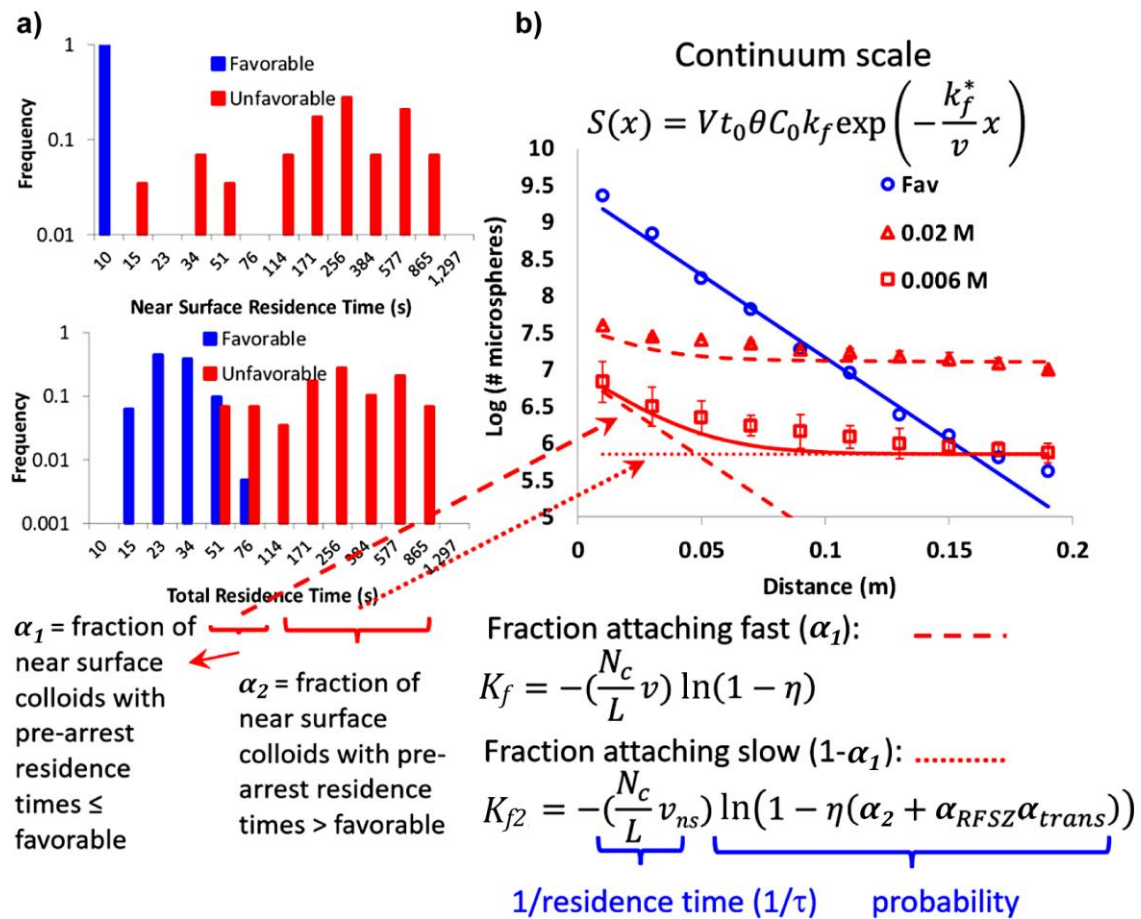
Figure 49 - a) Residence time distributions from pore-scale trajectory simulations under the conditions of Li and others (2004) for carboxylate-modified polystyrene colloids in glass beads at 6 mM NaCl. b) Predicted retention profiles using attachment rate coefficients predicted from residence time distribution as implemented in the expression for S(x) (retained # of colloids).
