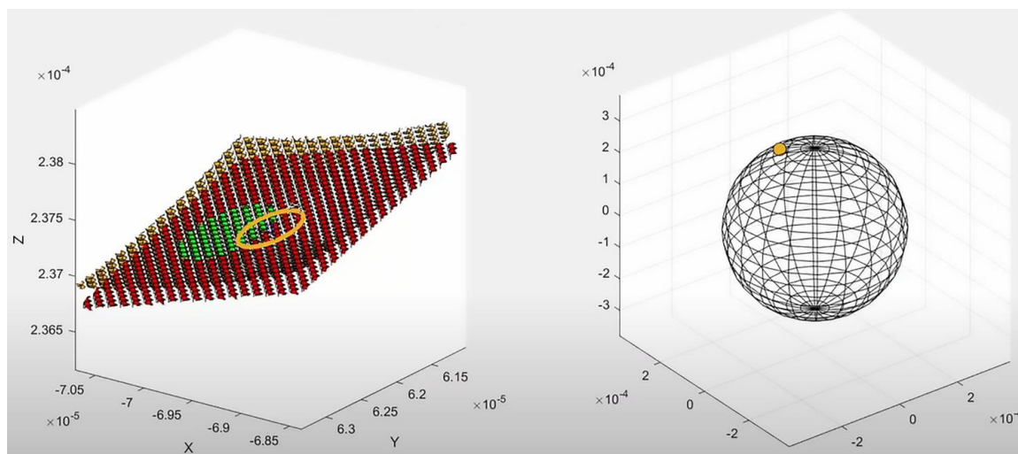
Figure 29 – A video introducing colloid detachment trajectory simulations using the Traj-Hap module's perturbation mode can be watched by clicking on the white arrow in the figure and the subsequent video symbol "▶" or clicking here: YouTube .
