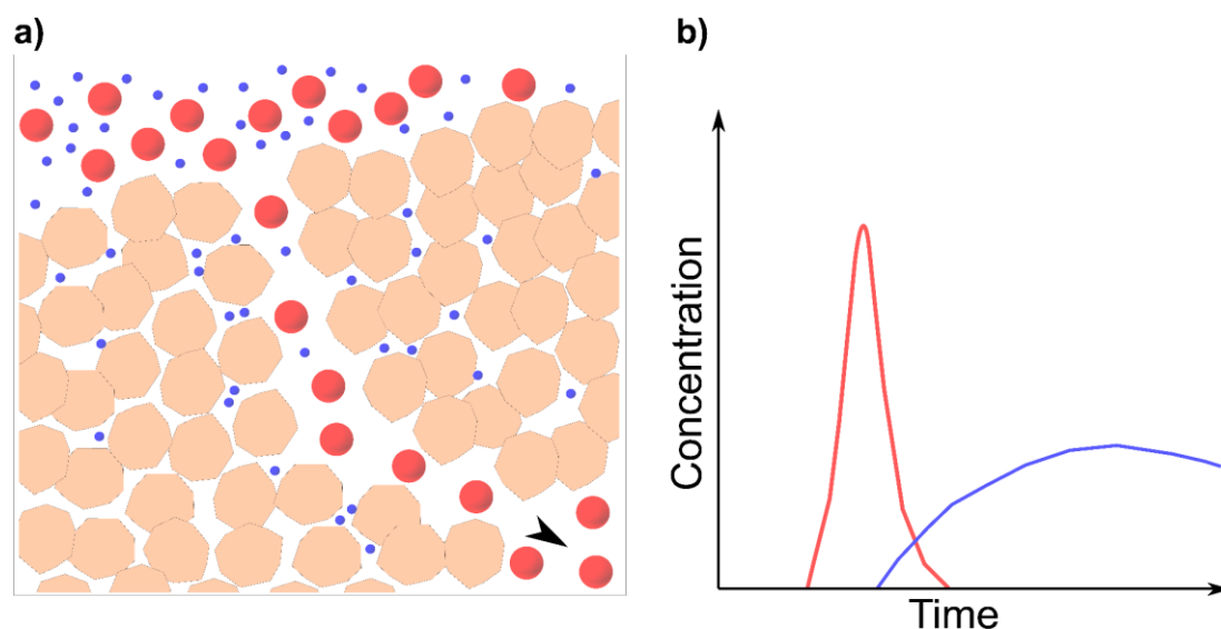
Figure 38 - Schematic of size exclusion of colloids relative to solutes in media with preferential flow. a) A preferential flow path through the host matrix. Larger colloids (red) are far less likely to enter the matrix porosity due to their relatively low diffusion (even when their physical size allows entry), thereby remaining in the higher velocity pore space. Smaller colloids (blue) have sufficiently high diffusion to enter the matrix porosity and experience slower fluid velocities. b) The resulting breakthrough-elution concentration histories demonstrate the resulting greater advection (arriving at earlier times) and lesser dispersion (the higher peak concentration) for colloids (red) relative to solutes (blue).
