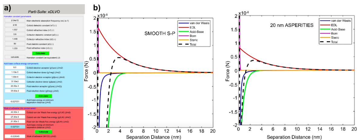
Figure 14 – The xDLVO module of Parti-Suite© with inputs shown in a) can be watched at this link YouTube and comparison of b) smooth surface behavior with behavior near a rough surface can be viewed here YouTube . The default inputs in the xDLVO graphical user interface (GUI) correspond to carboxylate-modified polystyrene latex microspheres interacting with glass slides across water and provide a specific example of the units used for these inputs.
