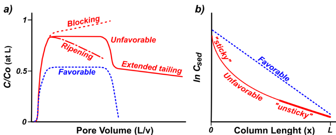
Figure 39 - a) BTC and b) RCP for step injection experiments for favorable (blue) and unfavorable (red) conditions. The behaviors labeled as blocking, ripening, extended tailing, sticky, and unsticky are explained in Section 6.2.
