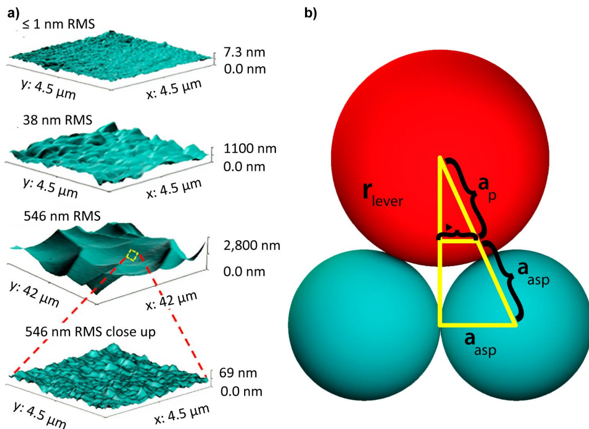
Figure 28 - Geometry of roughness a) surface topography revealed by atomic force microscopy for surfaces of three different root mean square (RMS) roughness. The fourth surface is a close-up of the 546 nm RMS roughness showing the fractal nature of roughness wherein smaller scale asperities occur on larger-scale asperities. b) Schematic of the geometric relationship used to determine the arresting lever arm ( r_{\text{lever}} ) resulting from contact with multiple asperities based on colloid and asperity radii of curvature ( a_p and a_{\text{asp}} , respectively).
