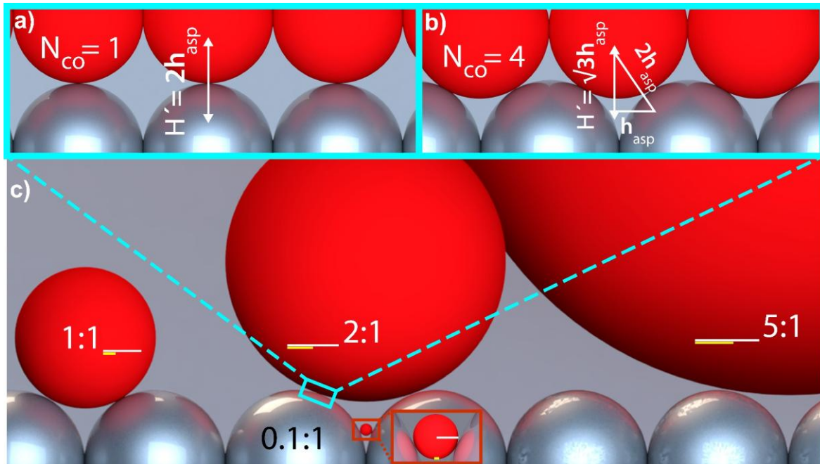
Figure 13 - Schematic showing geometries for hemispheres representing roughness asperities on colloid (red) and grain (metallic silver) surfaces in a) opposed (simple cubic packed, N_{co} = 1 ) and b) complementary (dense packed, N_{co} = 4 ) configurations. c) Colloids (red) achieving a contact area (radius shown by bold horizontal yellow line) with asperities on grain surface (metallic silver) relative to a lever arm defined by multiple contacts established as a function of the colloid:asperity ratio (white horizontal line). Colloid:asperity ratios are shown in the white text. Contact radii for the CML glass system were approximately 10 percent of the colloid radius. Calculations for the separation distance ( H' ) between the equivalent smooth surfaces located at asperity minima are shown in (a) and (b). The inset and its magnified view are shown for a 0.1:1 colloid:asperity ratio (modified from Rasmuson et al., 2019a).
