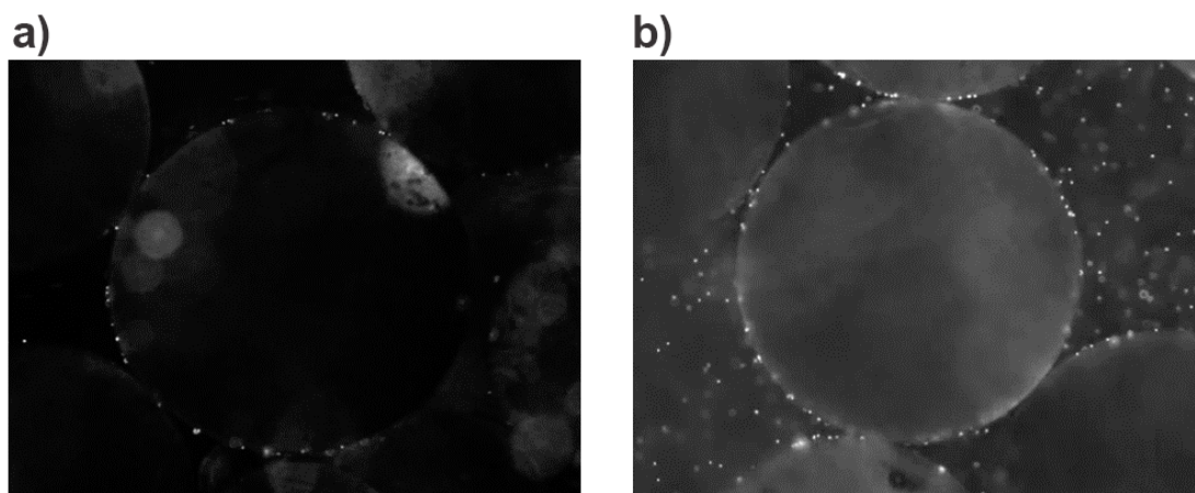
Figure 16 - Direct observation of colloid (fluorescent carboxylate-modified polystyrene latex microspheres of 2 \mu\text{m} diameter) transport in a microscopic granular media domain (glass beads of approximately 1 mm diameter). The main flow direction is from bottom left to top right. Colloids show as bright white dots. For favorable conditions shown in video a) , attachment occurs immediately once the colloid enters the near-surface fluid domain; there is no action at the grain surface other than the sudden appearance of the attached colloid. In contrast, for unfavorable conditions shown in video b) , colloids spend a significant time in the near-surface fluid domain prior to attachment or re-entrainment back to bulk fluid; there is frequent slow colloid motion along the grain surface, with a subset of the colloids becoming attached.
