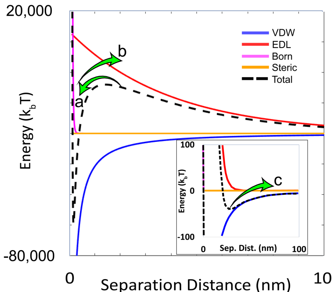
Figure 35 - Interpreting xDLVO profiles in terms of "label a" overcoming an energy barrier to attach in a primary minimum, and "label b" overcoming an energy barrier to detach from a primary minimum, and "label c" overcoming an energy barrier to re-entrain from secondary minimum. The VDW interaction increases via power law with decreasing separation distance such that it steepens similarly despite the vastly different y-scales in the inset and main figures.
