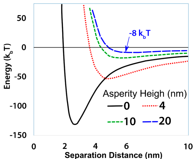
Figure 12 - Interaction energy profiles for 2 \mu\text{m} colloids under favorable conditions. Interactions for a smooth surface (i.e., no asperities present) are shown as a black line and interactions with 4 nm, 10 nm, and 20 nm asperities are shown with stippled red, dash-dot green, and dashed blue lines, respectively. Favorable conditions (pH 2, 50 mM) were calculated using \zeta_{\text{colloid}} = -5.1 \text{ mV} and \zeta_{\text{collector}} = 10.0 \text{ mV} .
