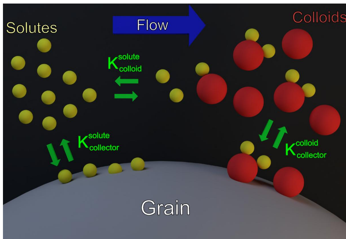
Figure 6 - Multiple interactions between dissolved solutes and suspended colloids, and each of them with grain surfaces. Constants for equilibrium partitioning of solutes and colloids with the grain surface and with each other are denoted with K_{ij}^i where i and j are the interacting moieties.
