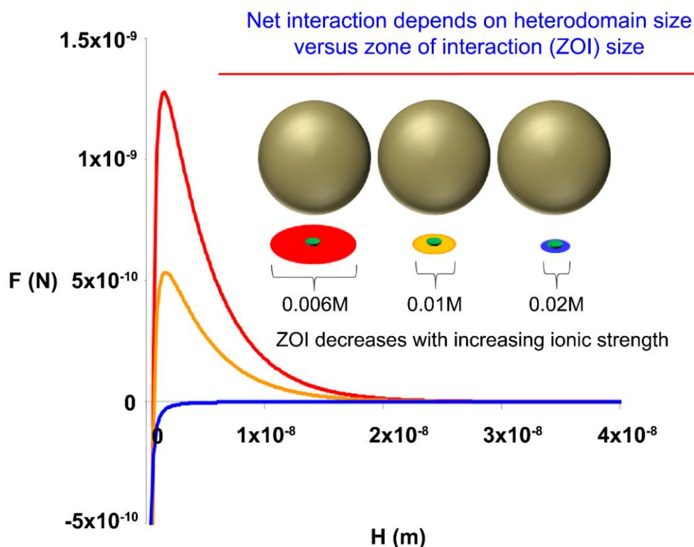
Figure 11 - Colloid–heterodomain interactions as a function of ionic strength. Colloids are depicted as gold spheres interacting with an underlying implied surface across a zone of interaction (ZOI) depicted by red, yellow, and blue disks. For a given size colloid ZOI is inversely proportional in size to solution ionic strength (IS). The area of charge heterogeneity on the surface is depicted as a green disk. The greater the fraction of ZOI occupied by heterodomain, the lesser the repulsive barrier as depicted by force profiles ( F ) versus colloid–surface separation distance ( H ) using colors (red, yellow, and blue) for the ZOI of the three colloid sizes. Positive values of F are repulsive, while negative values are attractive.
