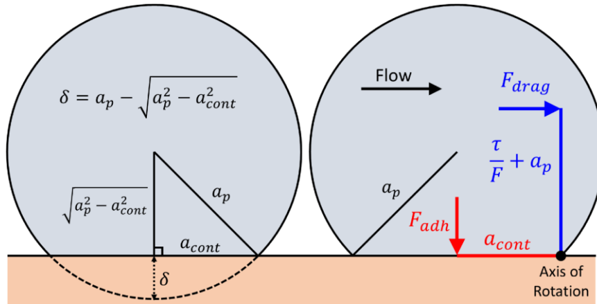
Figure 27 - Conceptual figure showing the deformation (left) and torque balance (right) applied to the colloid in contact with the collector surface.
