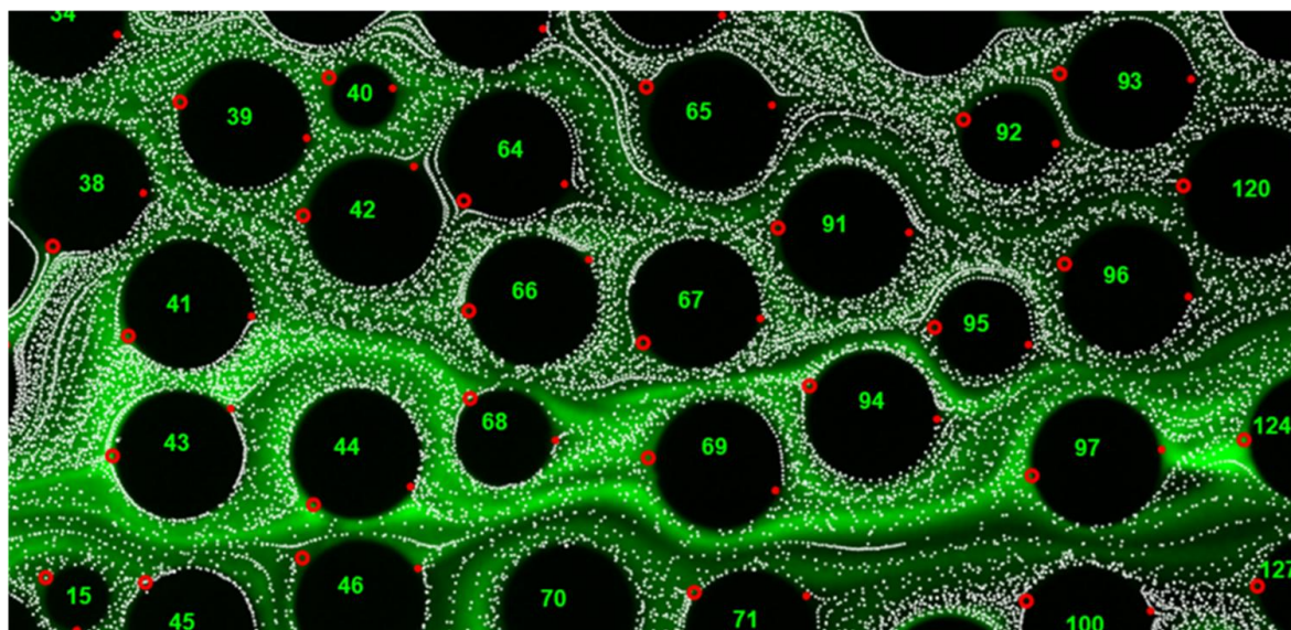
Figure 53 - Overlaid fluorescein (green brightness increases with concentration) and colloid trajectories (bright white) in 2D flow cell (50% porosity) and flow left to right. Open and closed red symbols show FFSP and RFSP, respectively. Image courtesy of Mr. Luis Ullauri.
