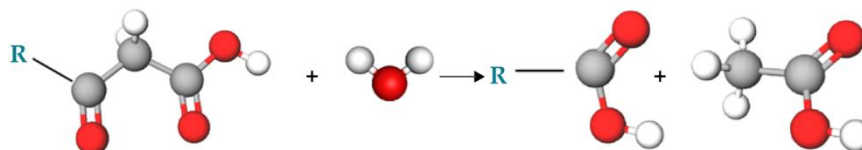
Figure 5 – Illustration of how \beta -oxidation stepwise oxidizes the \beta carbon (the C next to COOH) until it becomes a carboxylate group, with acetic acid ( CH_3COOH ) released by hydrolytic cleavage. R represents an organic group (e.g., a C chain or aromatic) attached to the \beta carbon; it is not altered by a round of \beta oxidation. Oxygen atoms are red.
