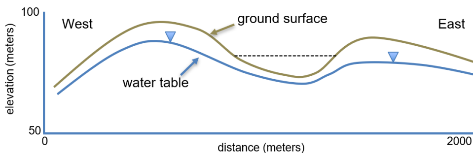
Figure Exercise 4-1 – Cross section of proposed tailings impoundment for Exercise 4.
