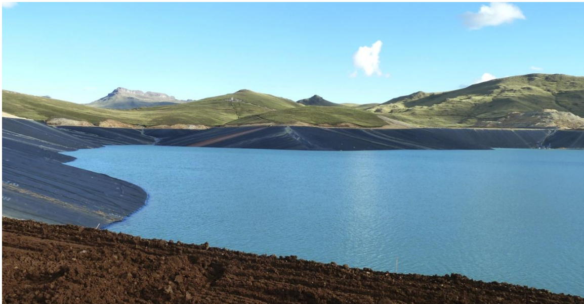
Figure 18 - Geomembrane liner installed in a tailings storage facility. At the time of this photograph, water was being accumulated in the facility for startup of mill operations.
